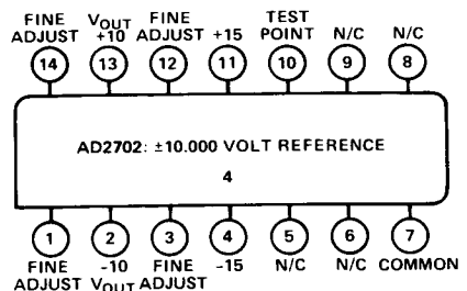
Device Type -5, -6
