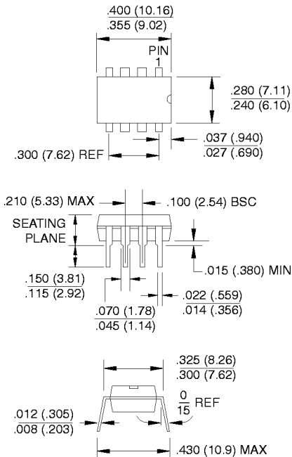
8P3 , 8-lead, 0.300" Wide, Plastic Dual Inline Package (PDIP) Dimensions in Inches and (Millimeters)
