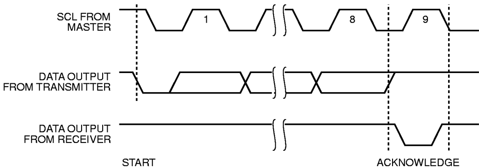
Figure 4. Acknowledge Timing
