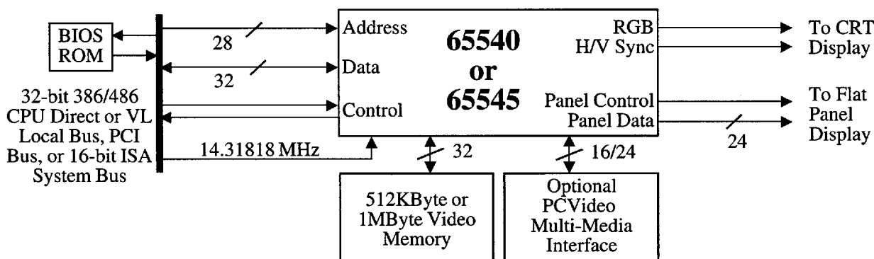
System Diagram
