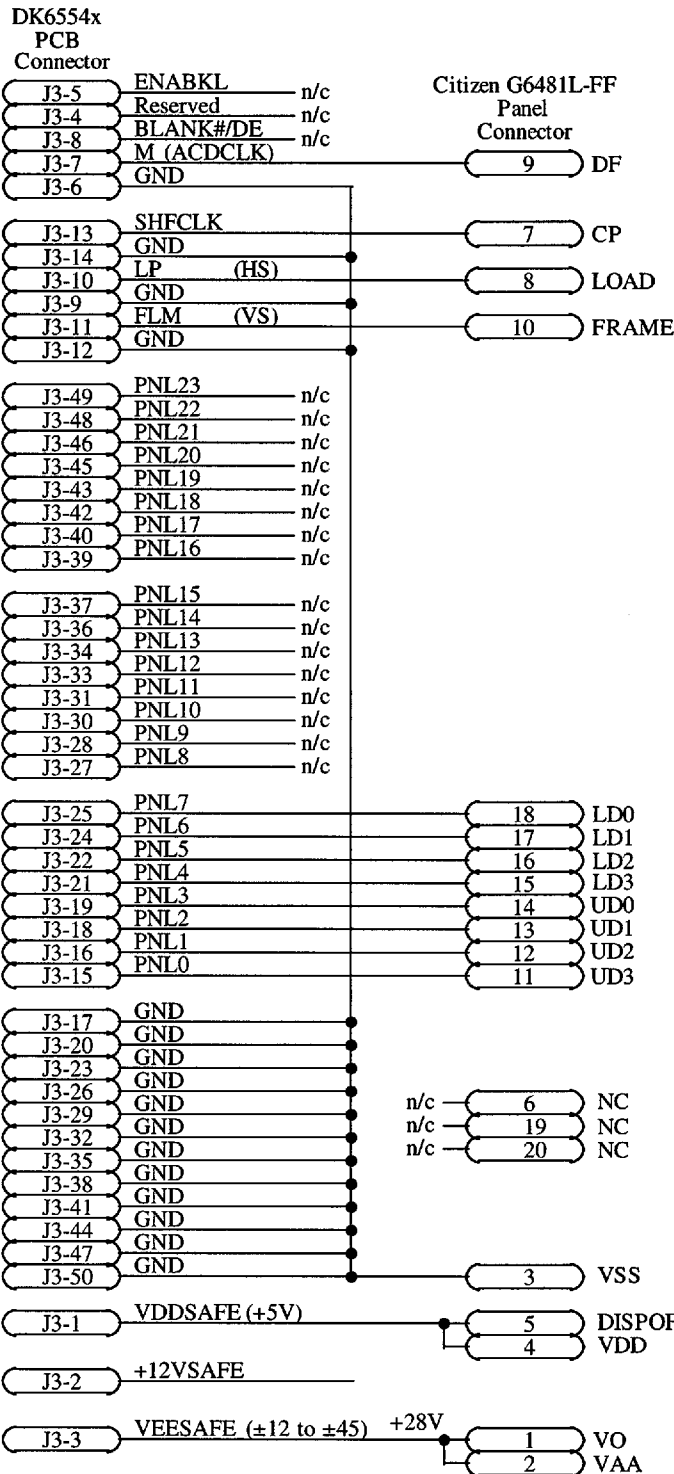
6554x Interface- Citizen G6481L-FF (640x480 Monochrome LCD DD Panel)
