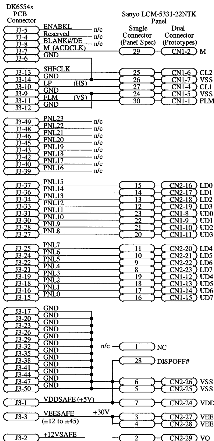
6554x Interface - Sanyo LCM-5331-22NTK (640x480 Color STN-DD LCD Panel)
