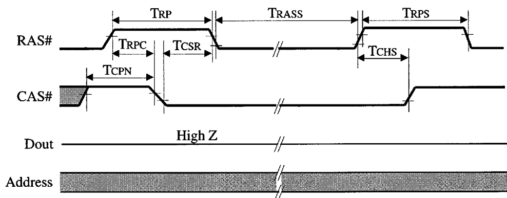
'Self-Refresh DRAM' Refresh Cycle Timing
