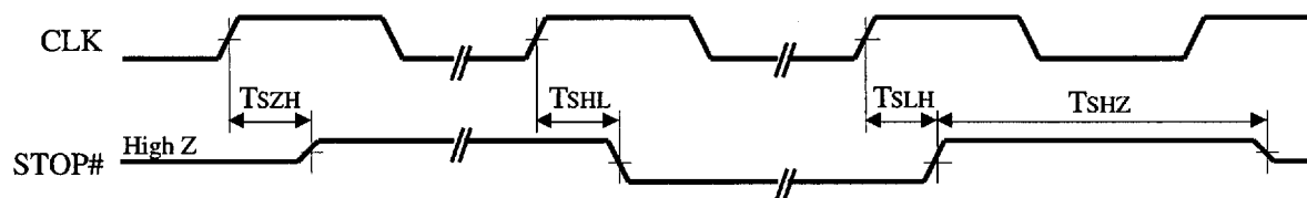
PCI Bus Stop Timing
