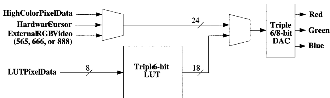
VGA Color Palette DAC Data Flow
