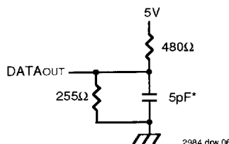
Figure 2. AC Test Load (for tCLZ, tCHZ, tWHZ, and tOW)
