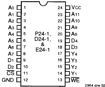
DIP/SOIC/SOJ/CERPACK TOP VIEW
