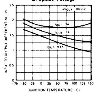
Dropout Voltage
