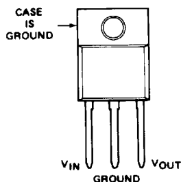
TO-218
