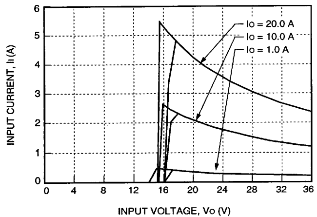
Figure 2. Typical JC100F Input Characteristics at Room Temperature
