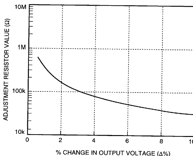
Figure 21. Resistor Selection for Increased Output Voltage
