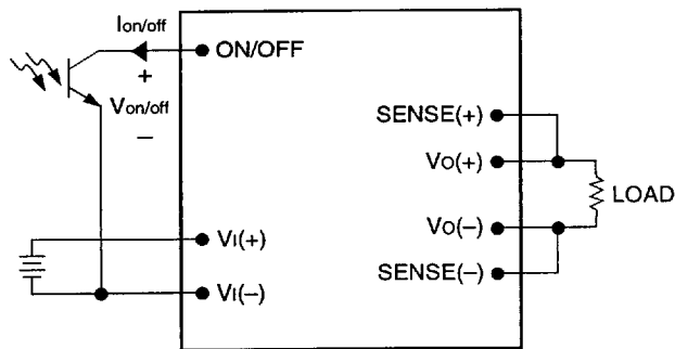
Figure 17. Effective Circuit Configuration for Single-Module Remote-Sense Operation
