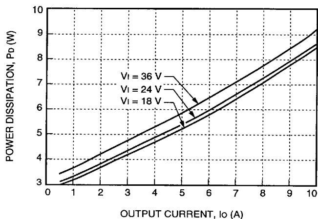
Figure 24. JC050F Power Dissipation vs. Output Current
