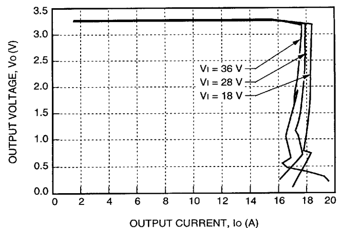
Figure 4. Typical JC075F Output Characteristics at Room Temperature
