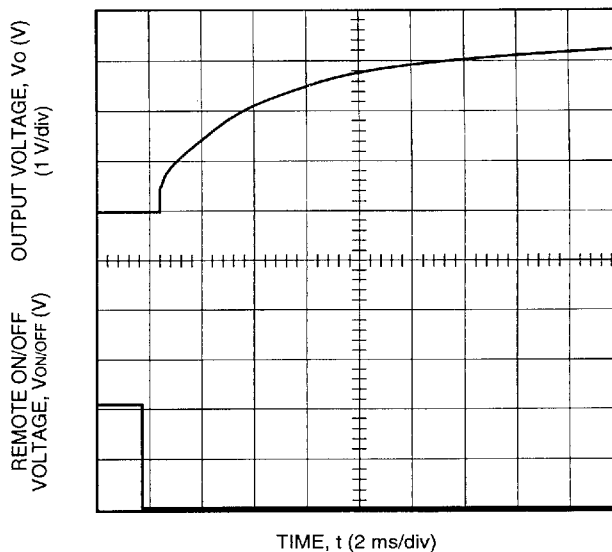
Figure 12. Typical Start-Up from Remote On/Off JC100F1; I_o = Full Load
