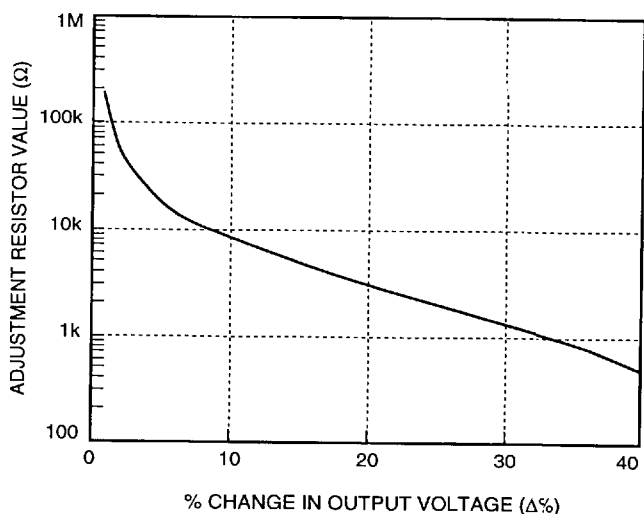
Figure 19. Resistor Selection for Decreased Output Voltage
