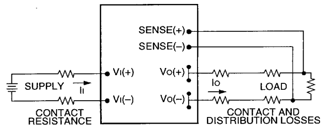
Figure 17. Effective Circuit Configuration for Single-Module Remote-Sense Operation
