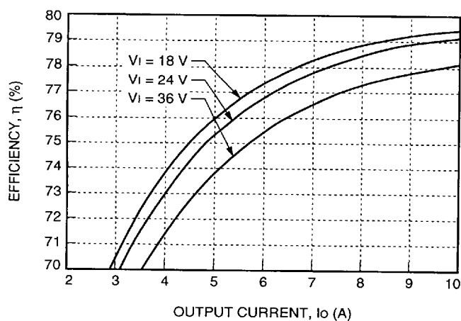
Figure 6. Typical JC050F Converter Efficiency vs. Output Current at Room Temperature
