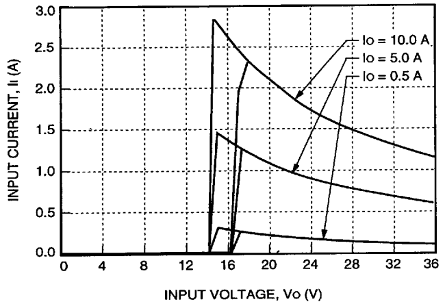
Figure 1. Typical JC050F Input Characteristics at Room Temperature
