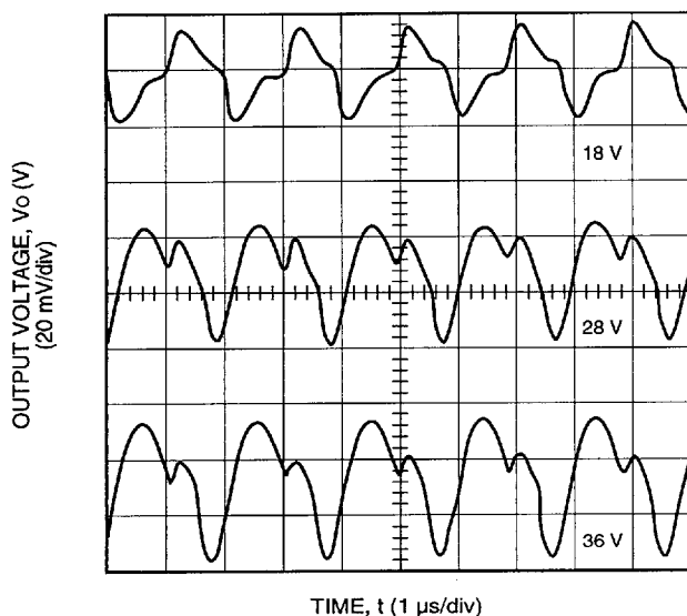
Figure 9. Typical JC100F Output Ripple Voltage at Room Temperature, and 20 A Output
