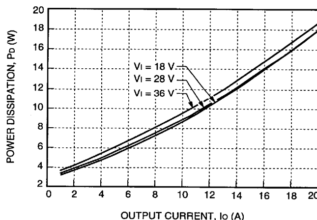
Figure 26. JC100F Power Dissipation vs. Output Current
