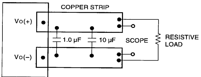
Figure 13. Input Reflected-Ripple Test Setup
