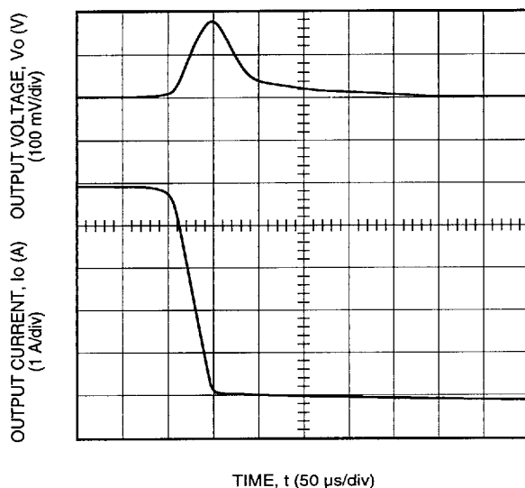
Figure 10. Typical JC100F Transient Response to Step Decrease in Load from 50% to 25% of Full Load at Room Temperature and 28 V Input (Waveform Averaged to Eliminate Ripple Component.)
