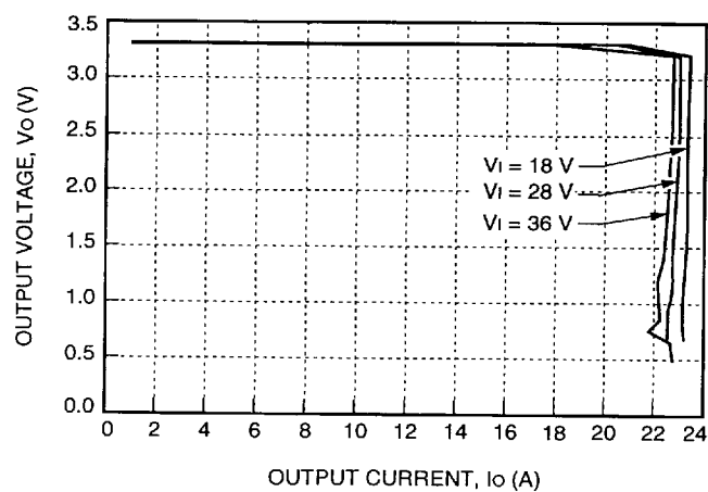
Figure 5. Typical JC100F Output Characteristics at Room Temperature
