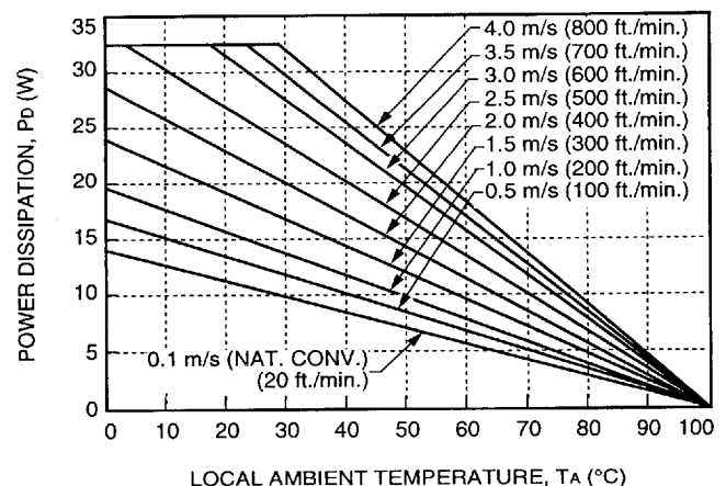
Figure 23. Forced Convection Power Derating with No Heat Sink; Either Orientation
