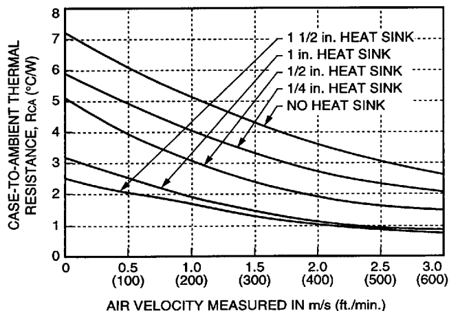
Figure 27. Case-to-Ambient Thermal Resistance Curves; Either Orientation
