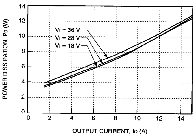
Figure 25. JC075F Power Dissipation vs. Output Current
