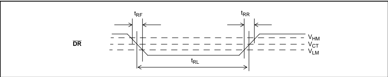
Figure 11 - DR Output Timing
