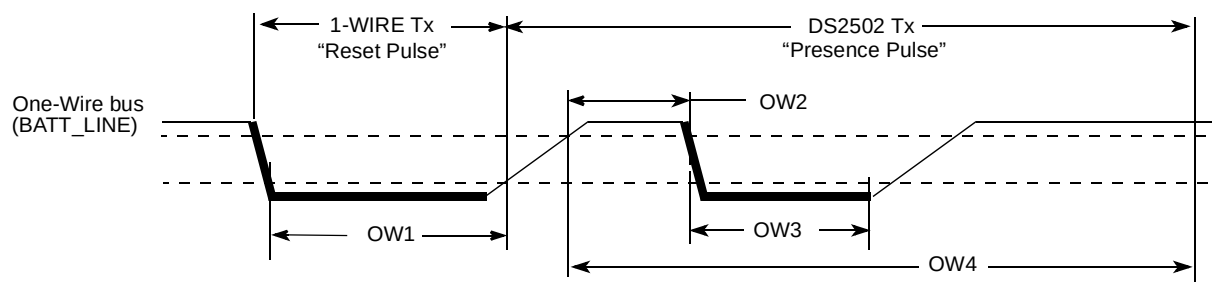
Figure 67. Reset and Presence Pulses (RPP) Timing Diagram
