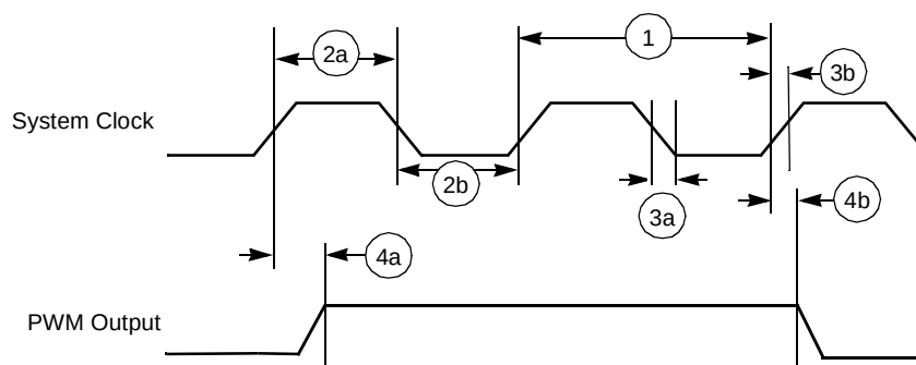
Figure 71. PWM Timing
