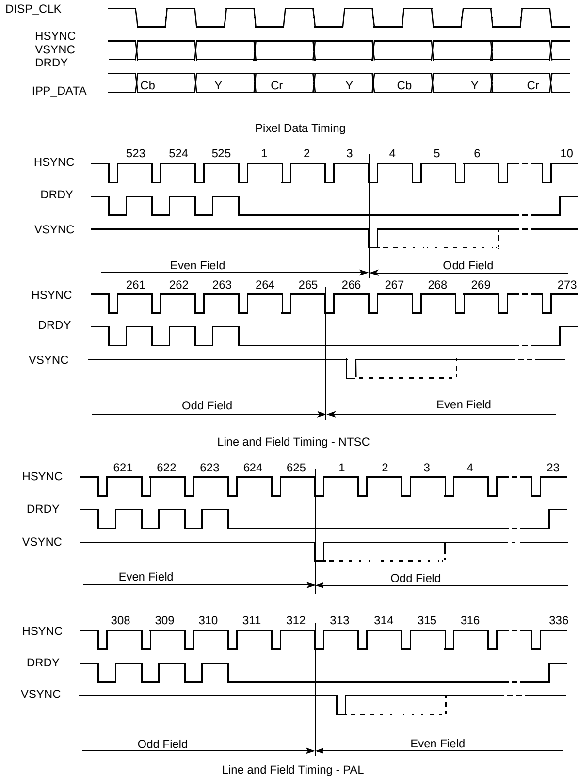
Figure 56. TV Encoder Interface Timing Diagram
