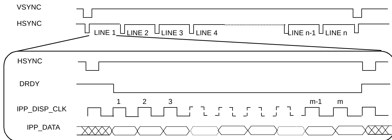
Figure 52. Interface Timing Diagram for TFT (Active Matrix) Panels
