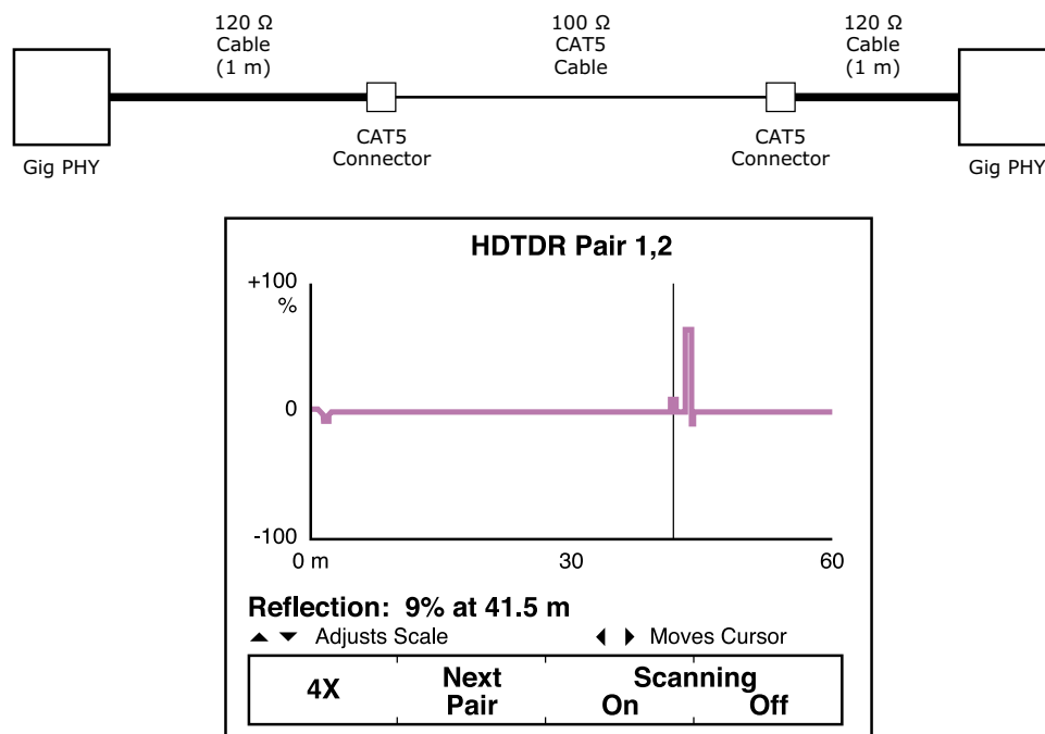
Figure 6: Gigabit Ethernet Impedance Mismatch Test Setup
