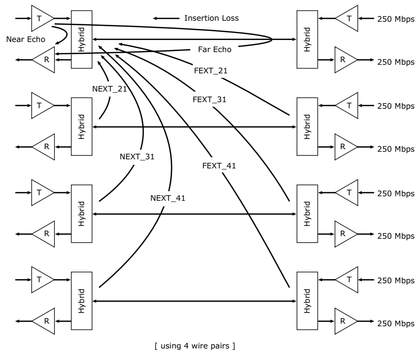
Figure 2: Sources of Noise in a Gigabit Ethernet System
