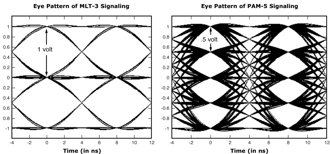
Figure 1: MLT-3 and PAM-5 Signal Levels
