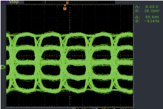
Figure 5: The Eye Diagram at 140 Meters Category 5 Cable Using the Marvell Alaska Gigabit PHY Transceiver
