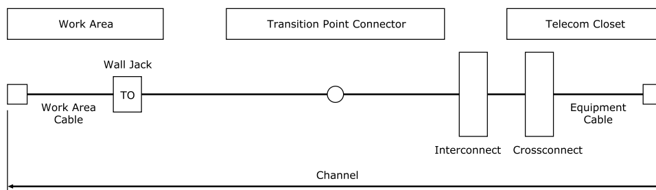
Figure 3: ANSI/EIA/TIA Horizontal Cabling Subsystem
