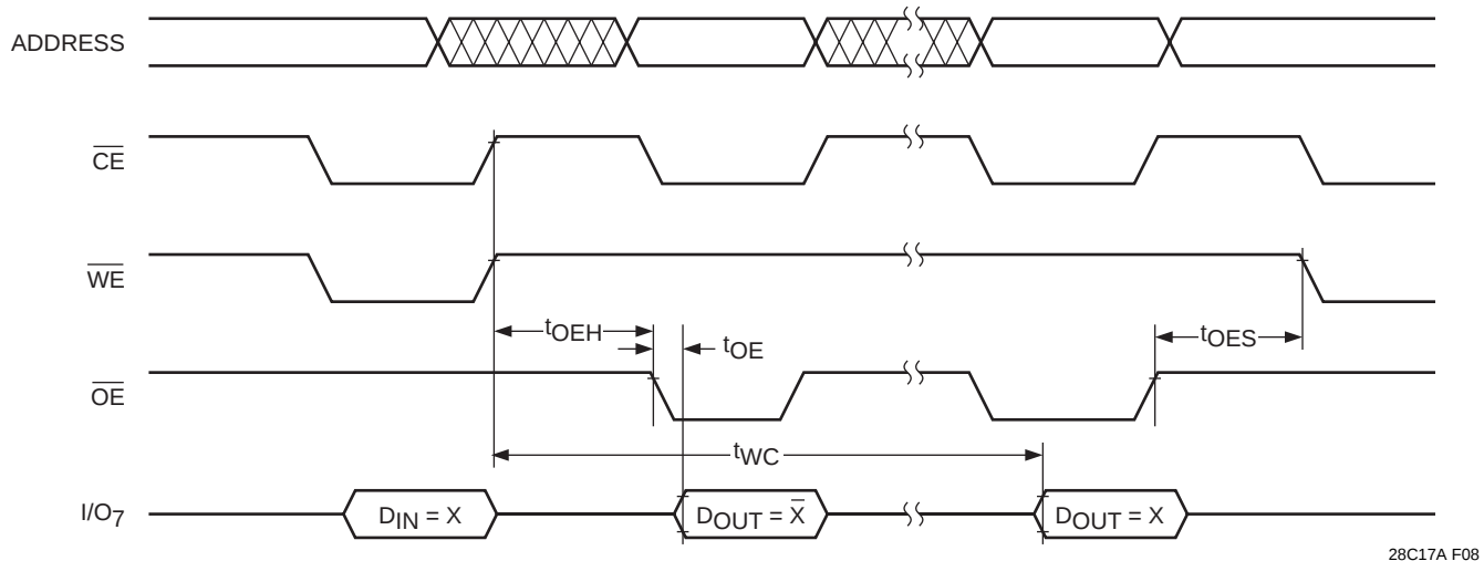
Figure 6. DATA Polling
