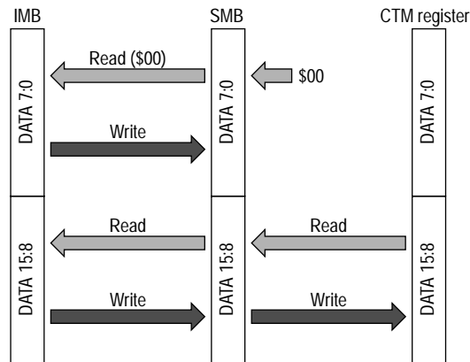
Figure 1-2 8-bit (byte) access (even addresses)
