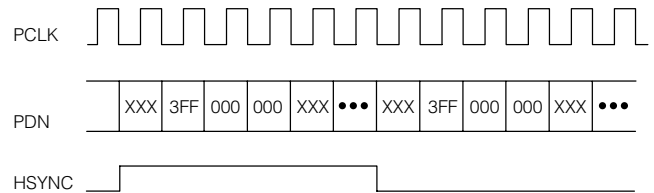
Fig. 10 Operation of HSYNC with Respect to PCLK
