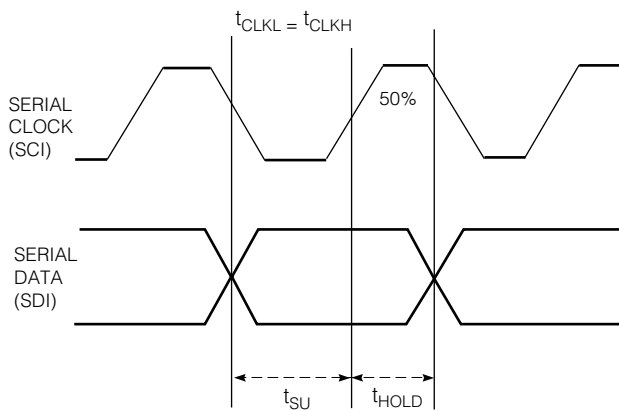
Fig. 7 Waveforms
