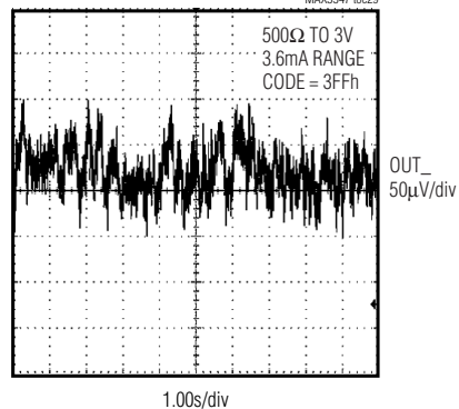
OUTPUT NOISE (0.1Hz TO 10Hz)
