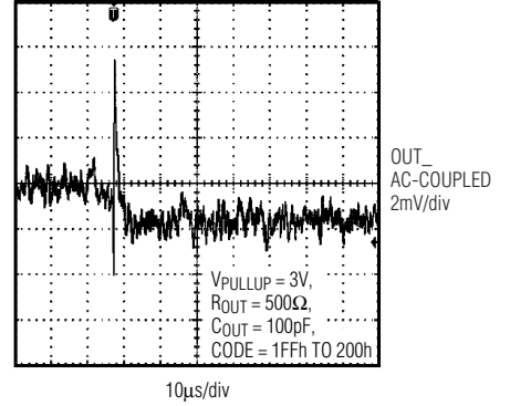
GLITCH IMPULSE (MAJOR CARRY TRANSITION) ( I_{OUT} = 3.6mA )
