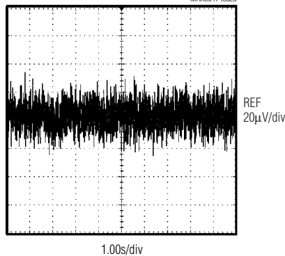
INTERNAL REFERENCE NOISE (0.1Hz TO 10Hz)
