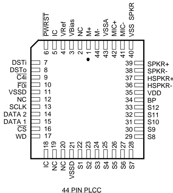
Figure 2 - Pin Connections
