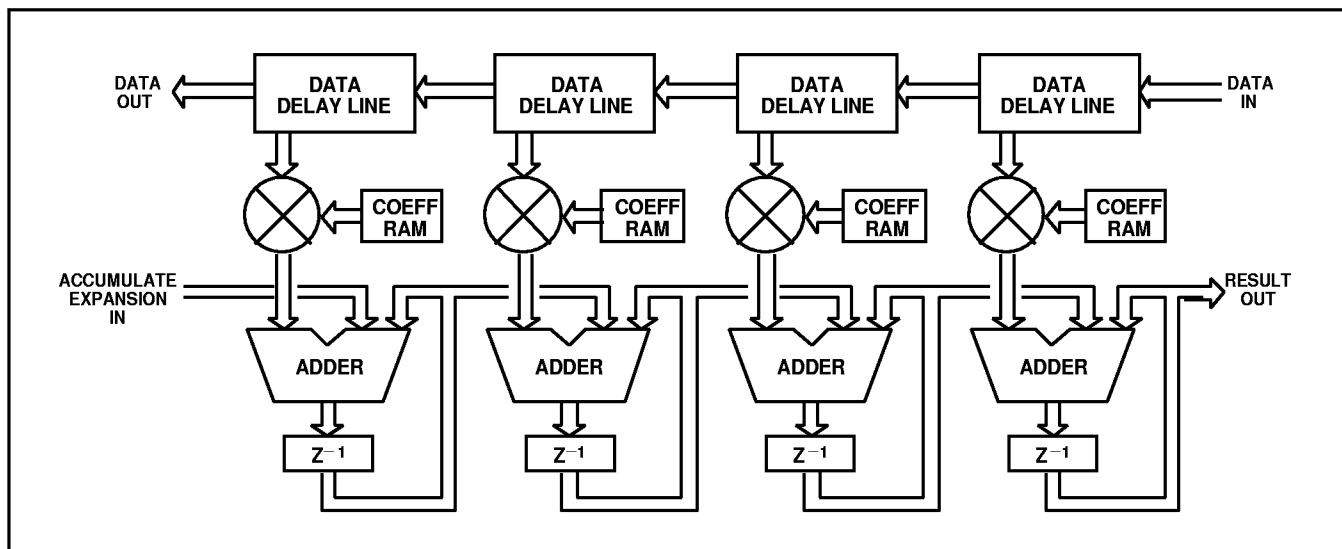
Fig. 4 Filter network diagram
