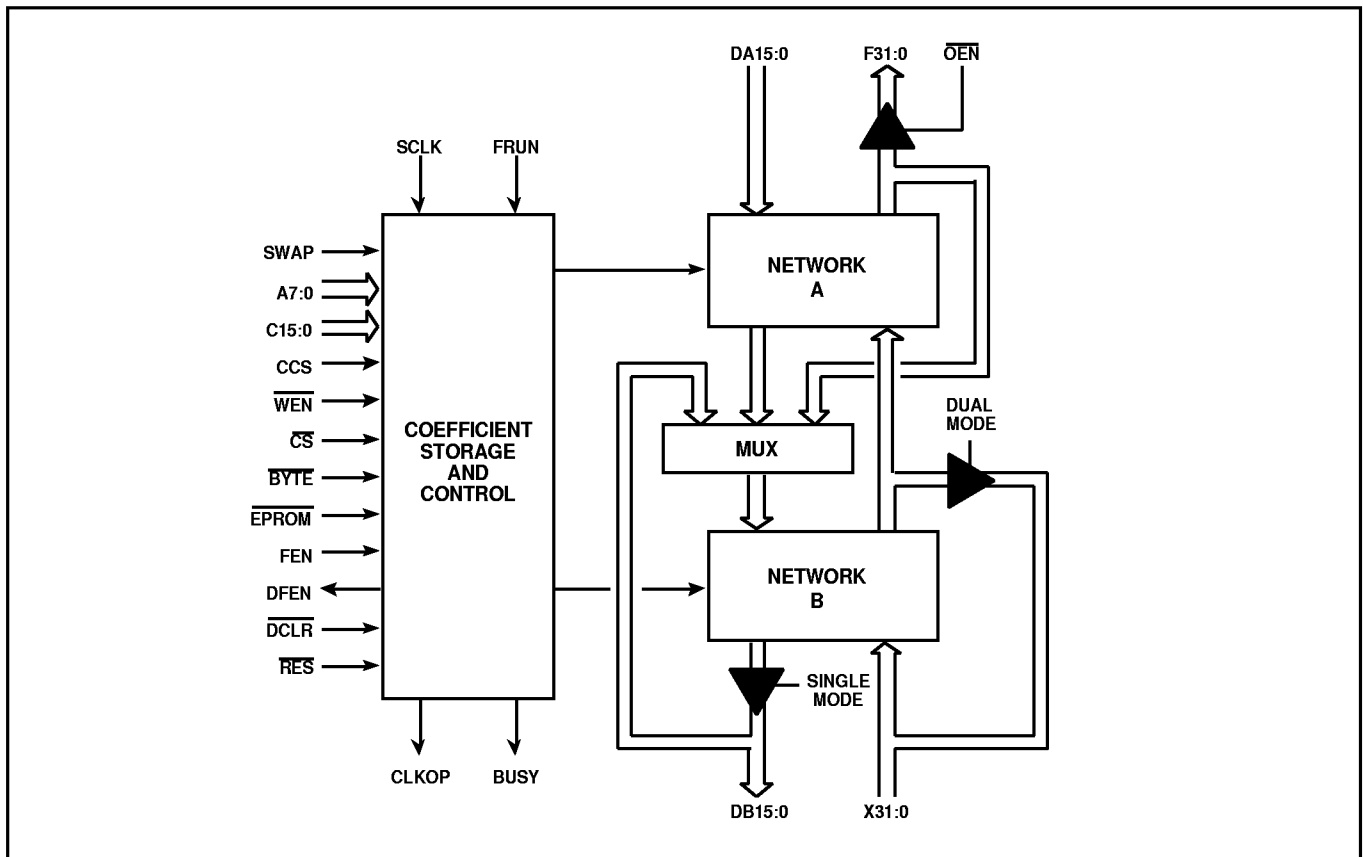
Fig. 3 Block Diagram
