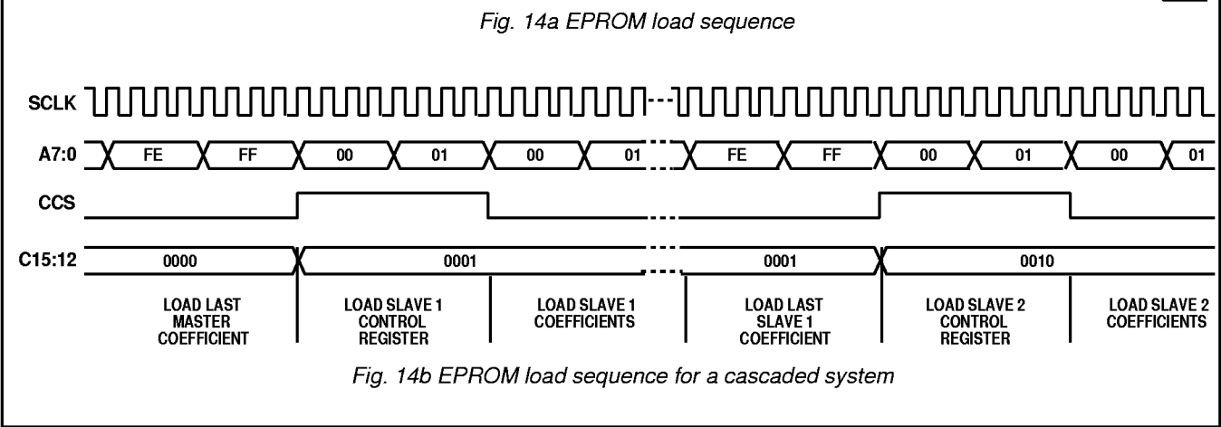
Fig. 14 EPROM load sequence timing diagrams
