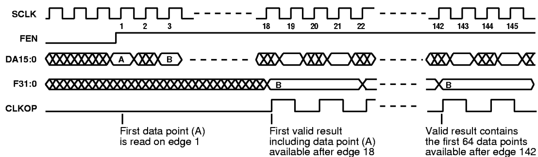
Fig. 6 Single Filter timing diagrams
