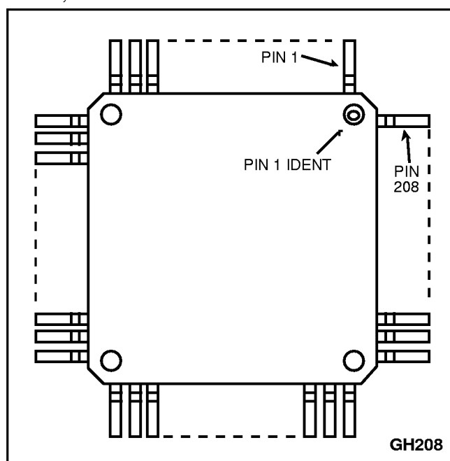
Pin identification diagram (top view)
