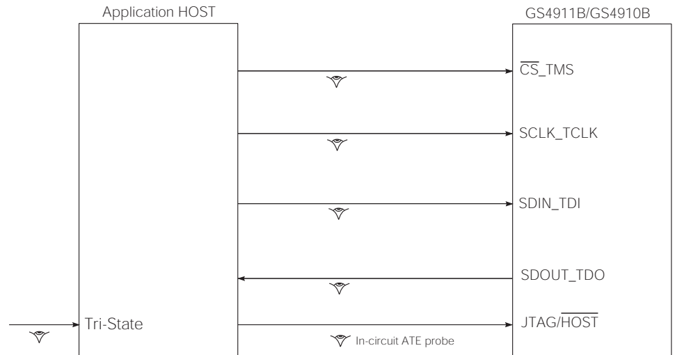
Figure 3-17: System JTAG
