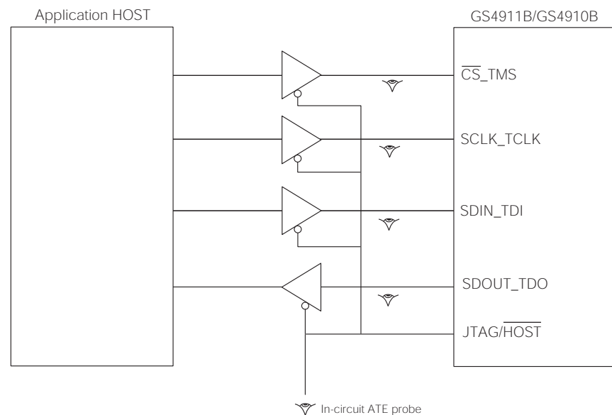
Figure 3-16: In-Circuit JTAG
