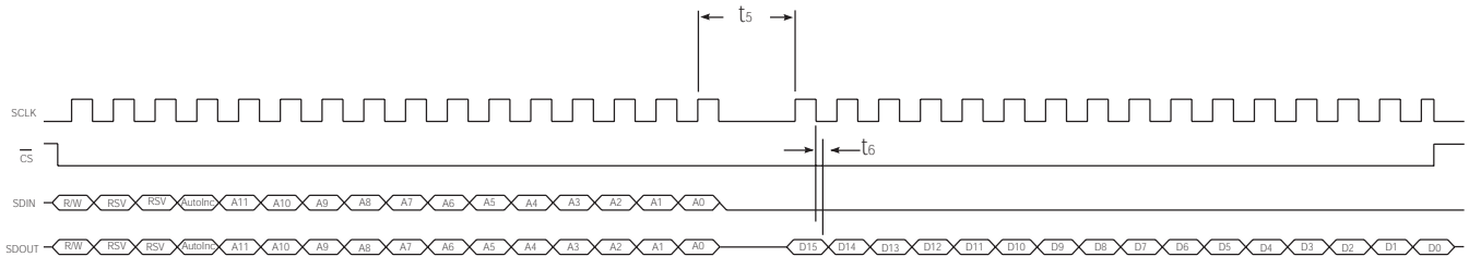
Figure 3-14: GSPI Read Mode Timing
