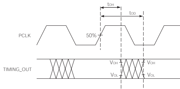
Figure 2-1: PCLK to TIMING_OUT Signal Output Timing
