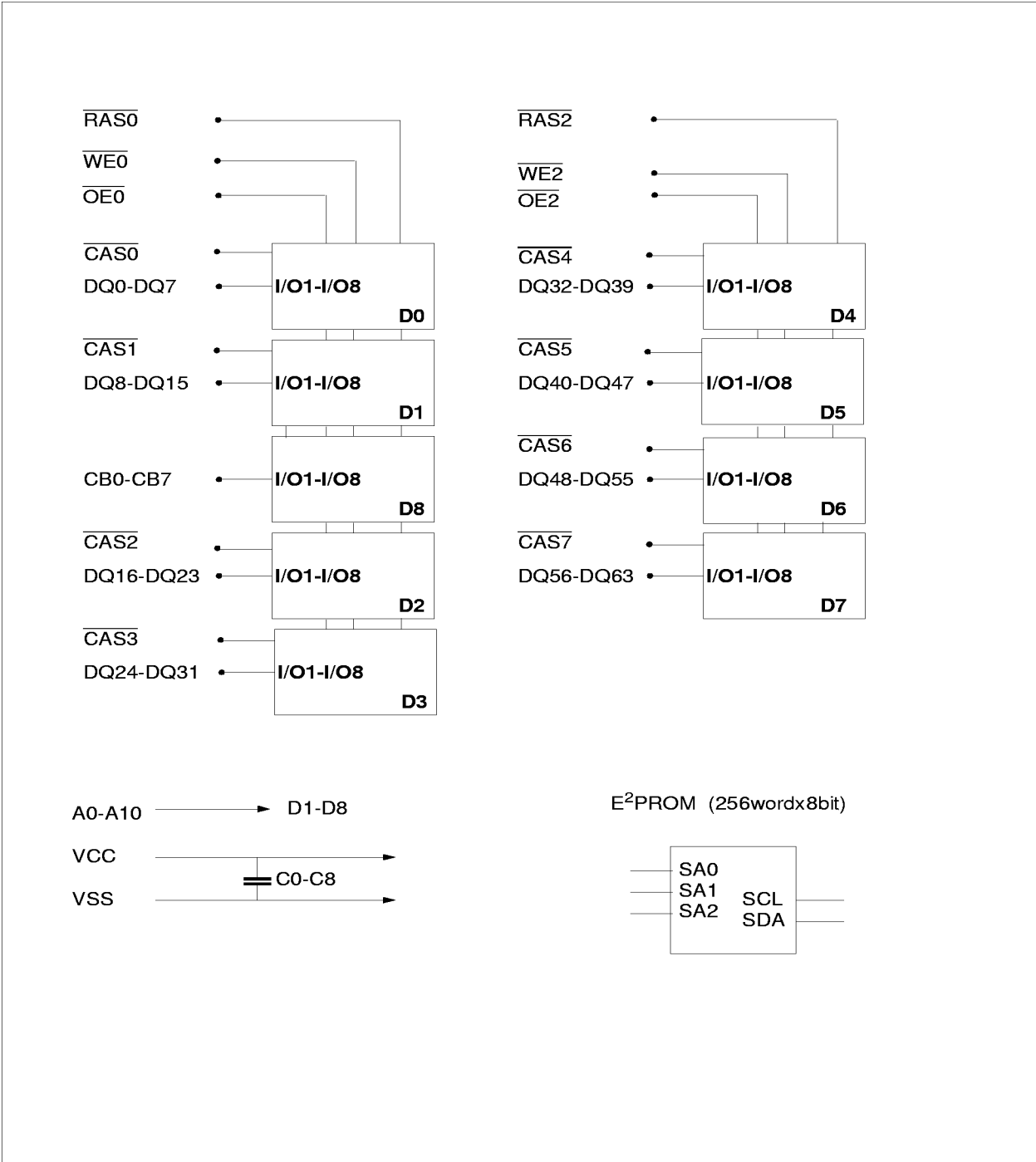
2M x 72 DIMM Module Block Diagram
