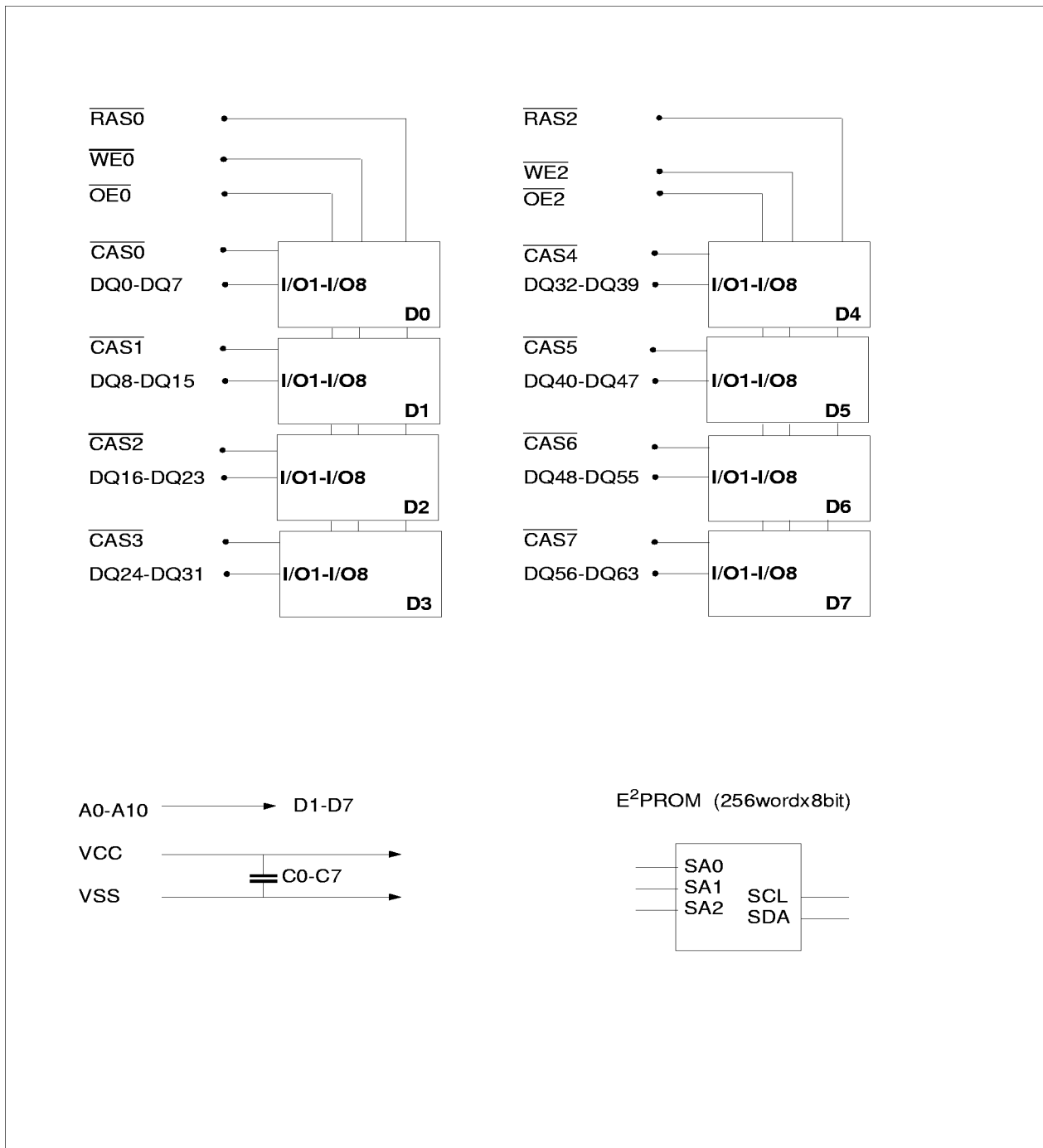
2M x 64 DIMM Module Block Diagram
