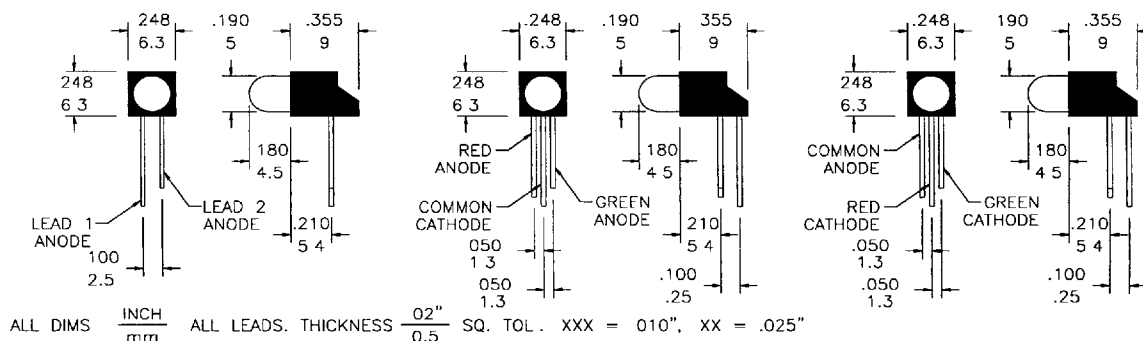
FIG 1 2-LEADED STD. & LOW DOME
