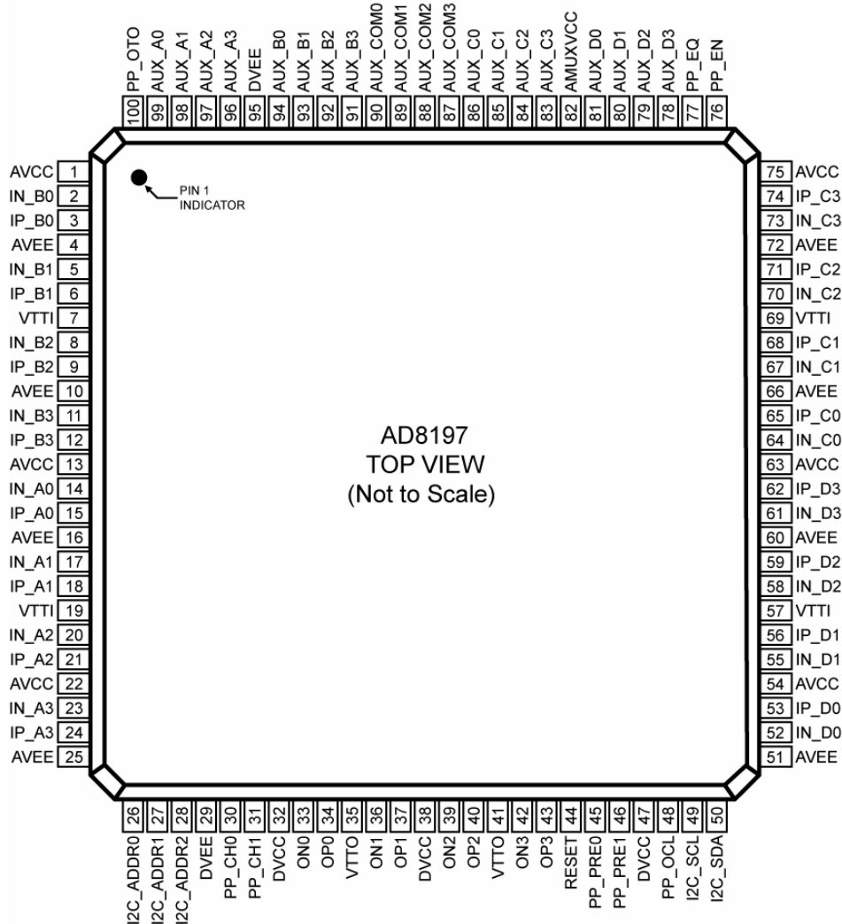
Figure 3. Pin Configuration
