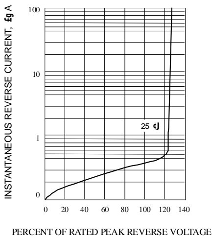
Fig. 3- REVERSE CHARACTERISTICS
