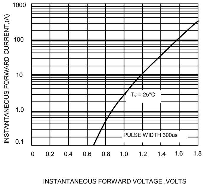
FIG.4-TYPICAL FORWARD CHARACTERISTICS
