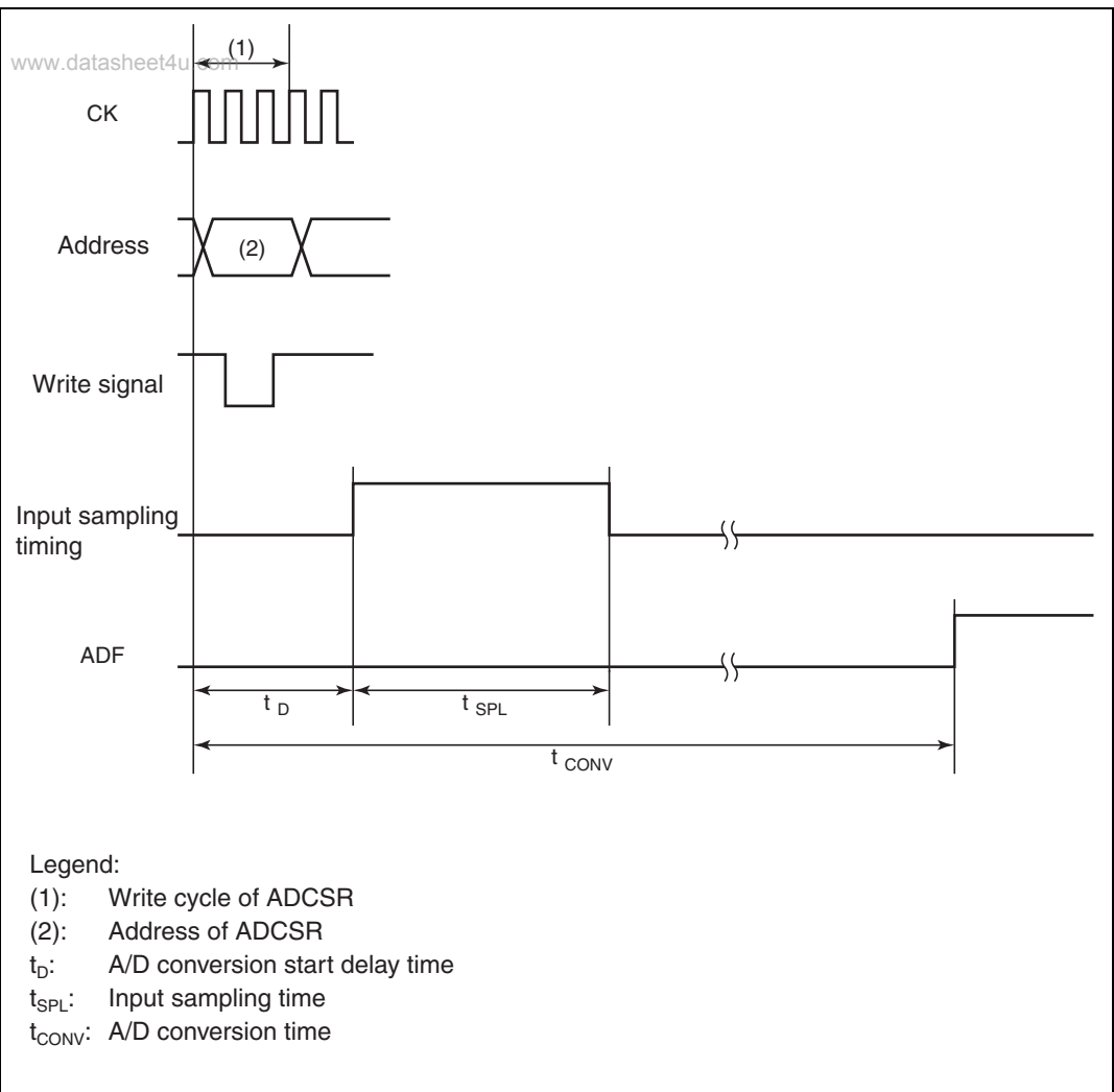
Figure 14.5 A/D Conversion Timing
