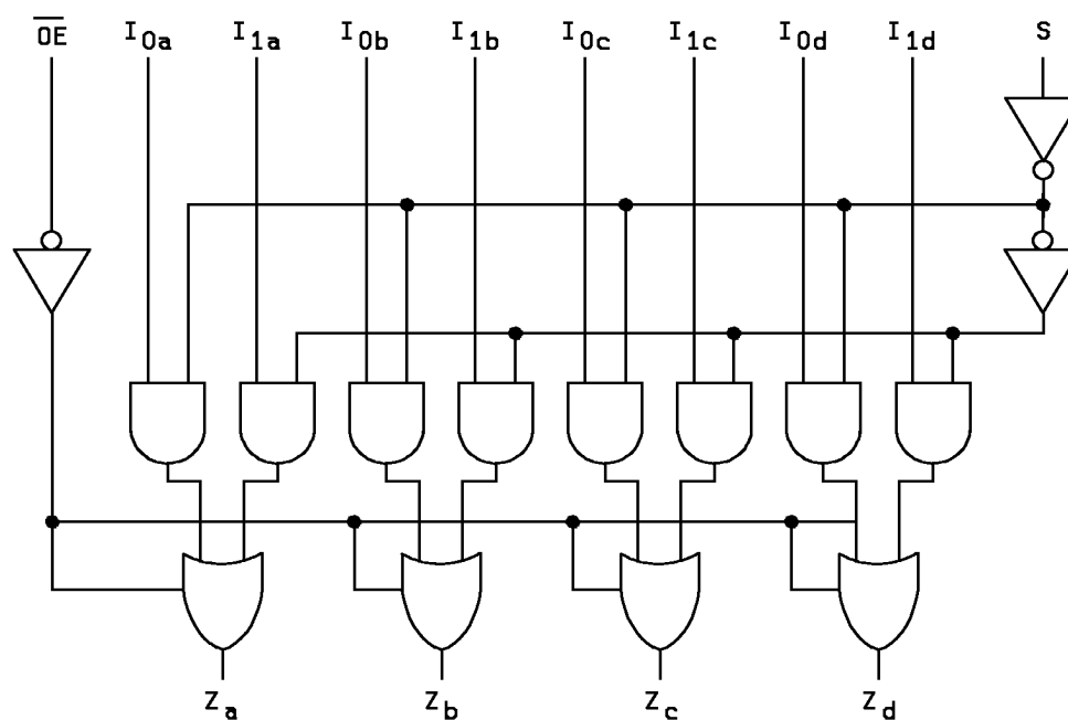
FIGURE 3. Logic diagram.
