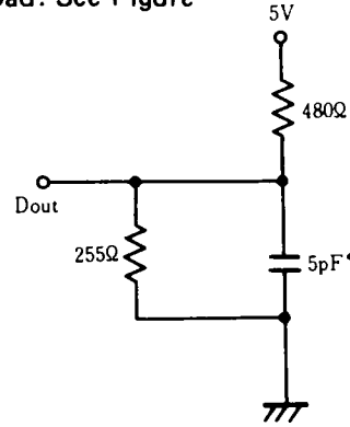
Output Load (B)
