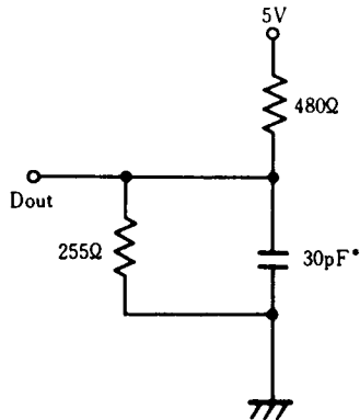
Output Load (A)
