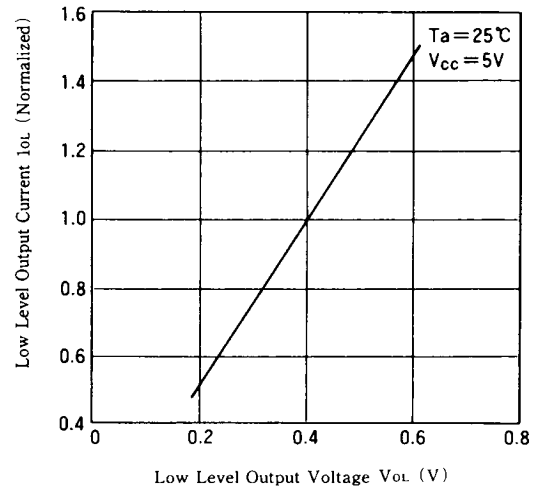
OUTPUT CURRENT VS. OUTPUT VOLTAGE(2)
