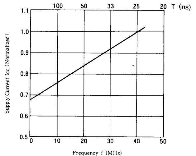
SUPPLY CURRENT VS. FREQUENCY
