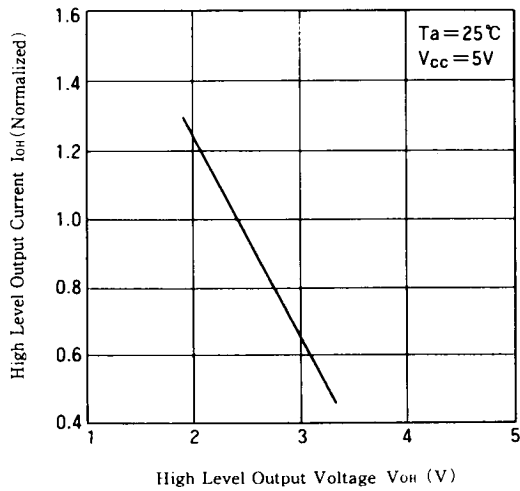
OUTPUT CURRENT VS. OUTPUT VOLTAGE(1)
