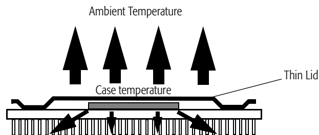
Figure 21. Processor's Heat Dissipation Path
