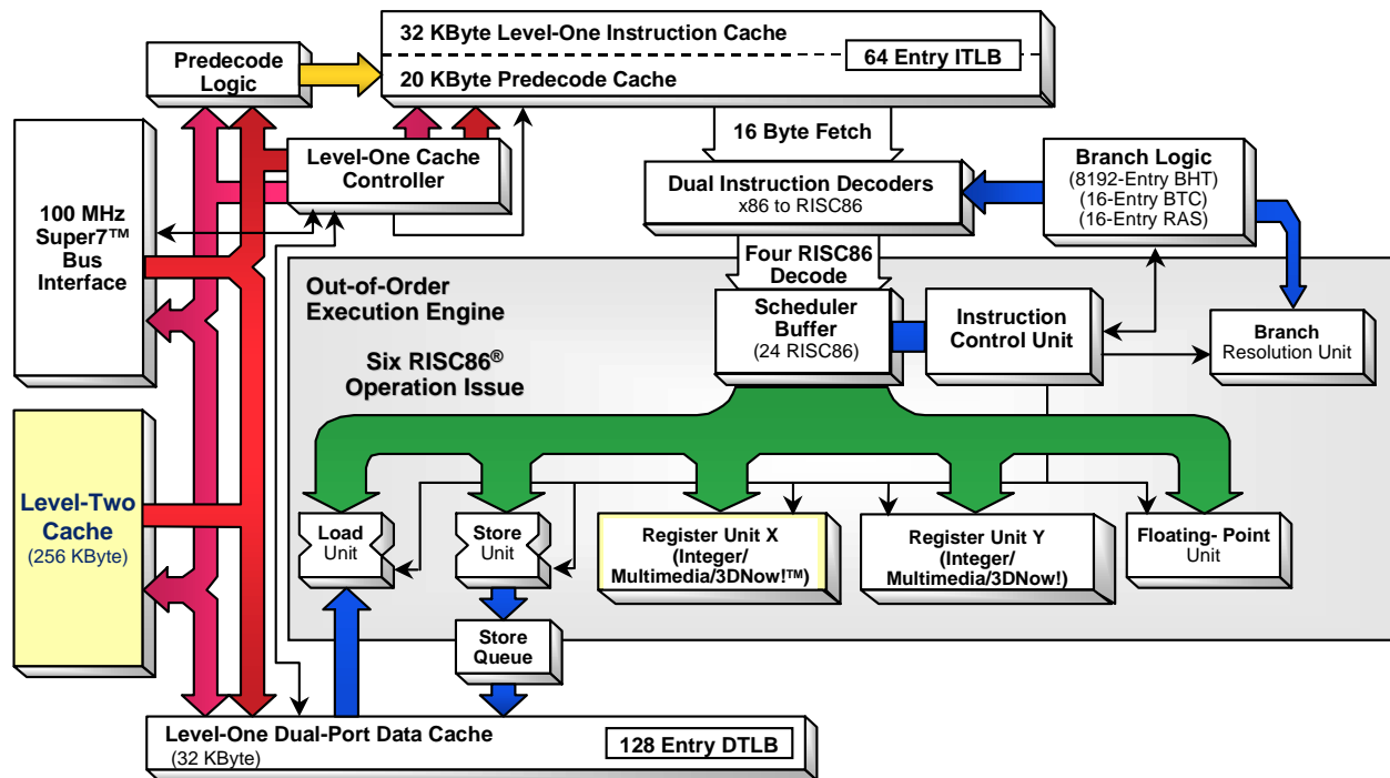
Figure 1. Mobile AMD-K6®-III-P Processor Block Diagram
