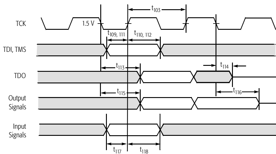
Figure 17. Test Signal Timing Diagram
