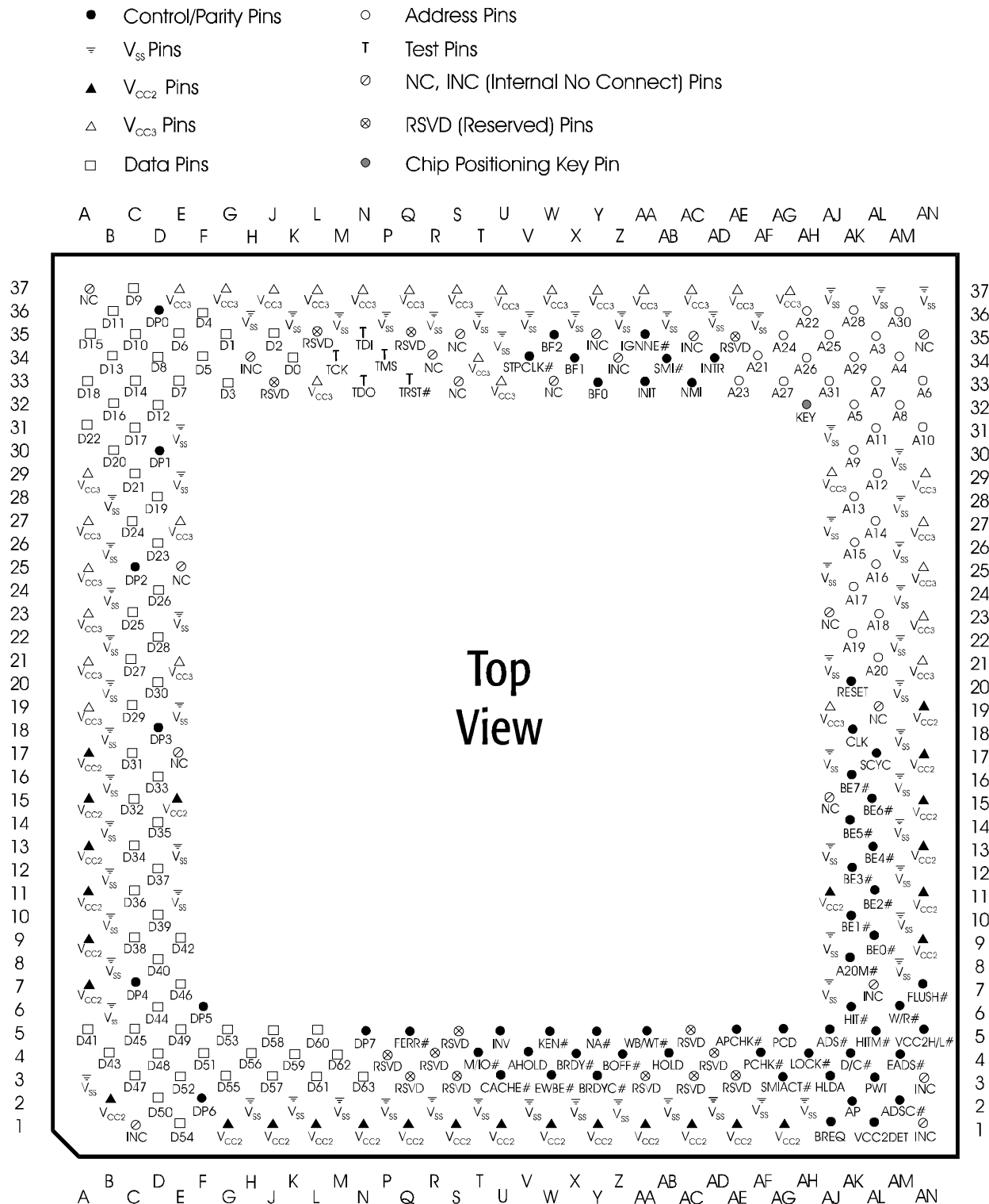
Figure 25. Mobile AMD-K6®-III-P Processor Top-Side View
