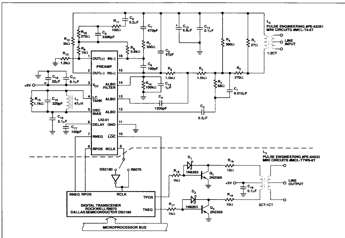
FIGURE 13: The LIU-01 enables this 4-wire transceiver to recover T1 data at 1.544Mbps/s with an input signal level varying from 0dB to less than -38dB. The ALBO/equalization network is compatible with unshielded #22AWG twisted-pair wire measuring 16pF/ft.
