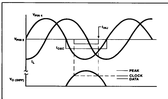
FIGURE 12: The LC tank is synchronized to the incoming data when the clock detector injection current, I_{INJ} , is centered inside the oscillator's bias current pulse.
