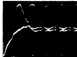
FIGURE 16: The LIU-01's preamplifier output, pin #1, should produce half-sinusoidal pulses of recovered data signal when properly equalized for the transmission line. The circuit of Figure 13 has excellent response as shown here receiving at 6000 ft. a 1-of-9 pattern, a, and a QRSS pattern, b.
