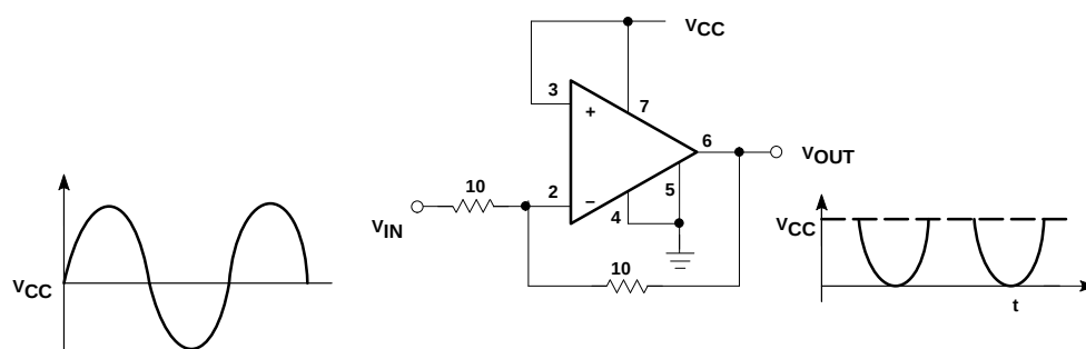
b. Negative-Going Output Referenced to V_{CC}
