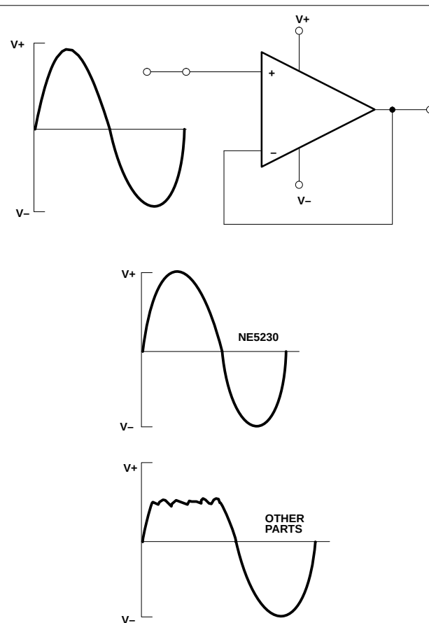
Figure 4. In a Non-Inverting Voltage-Follower Configuration, the NE5230 will Give Full Rail-to-Rail Swing. Other Low Voltage Amplifiers will not Because they are Limited by their Input Common-Mode Range and Output Swing Capability.
