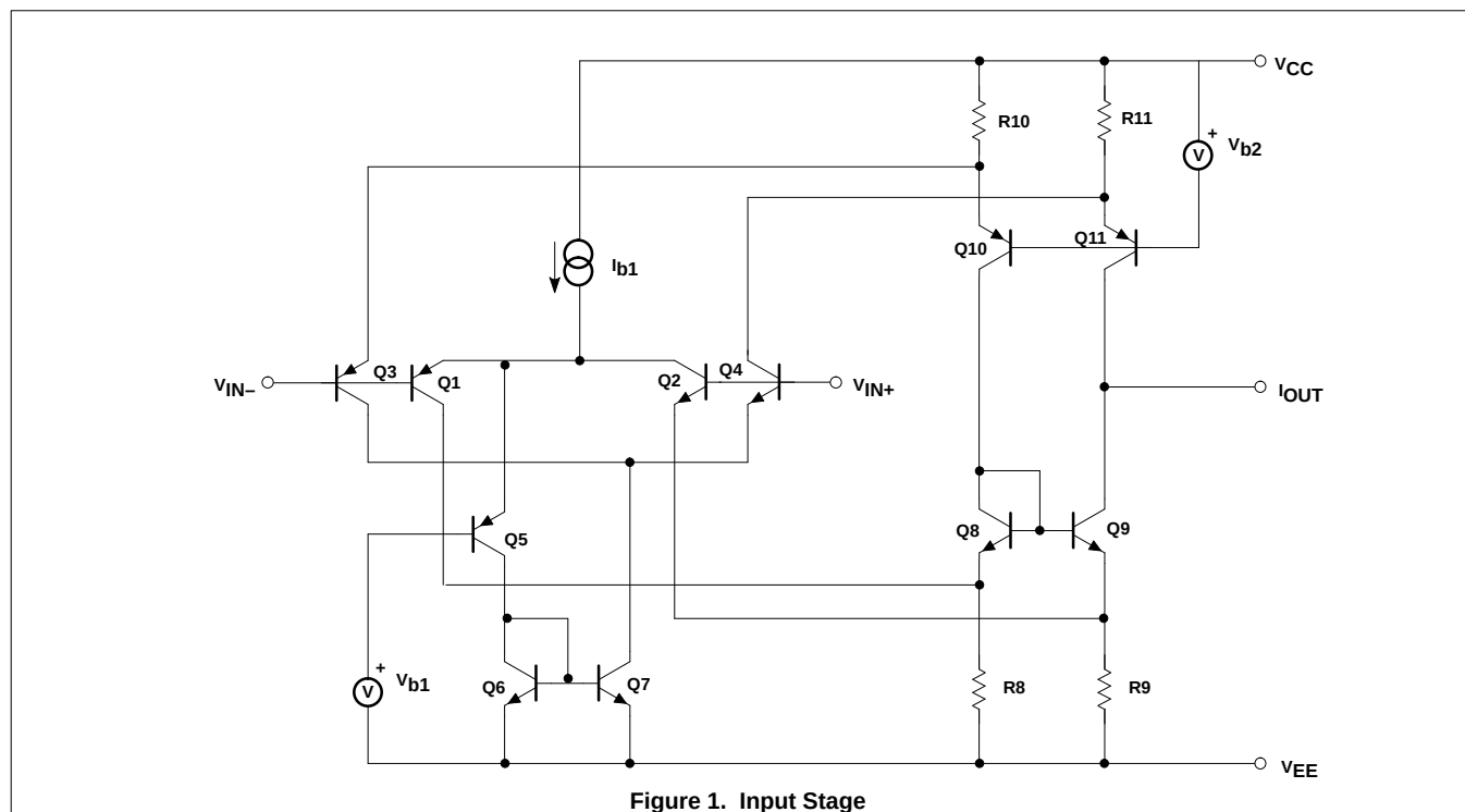
Figure 1. Input Stage
