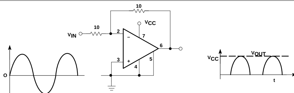
a. Rail-to-Ground Output Swing Referenced to Ground
