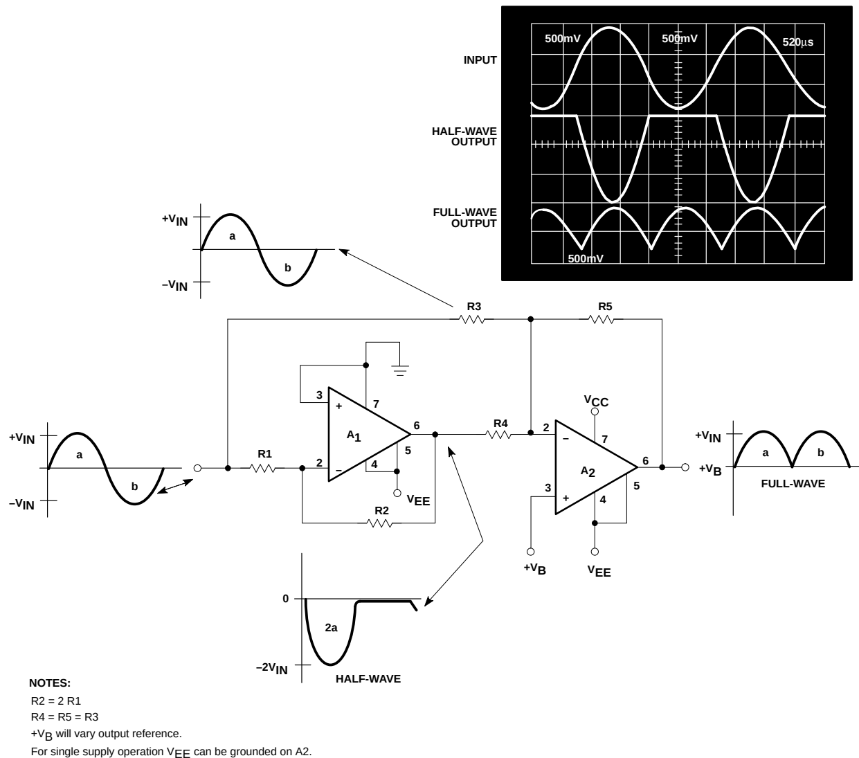
Figure 9. Adding an Inverting Summer to the Input and Output of the Half-Wave will Result in Full-Wave
