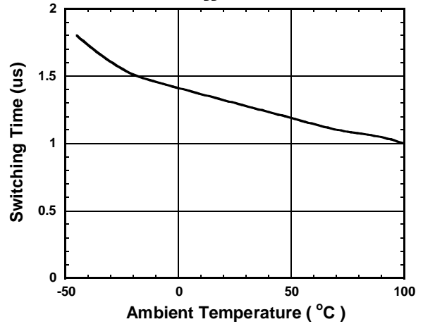
Switching Time vs. Ambient Temperature ( V_{DD}=2.85V )
