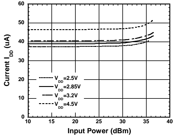
Current I_{DD} vs. Input Power ( f=0.9GHz, P1-P3 ON, CTL1=CTL2=0V )
