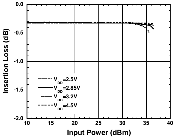
Insertion Loss vs. Input Power ( f=0.9GHz, P1-P3 ON, CTL1=CTL2=0V )
