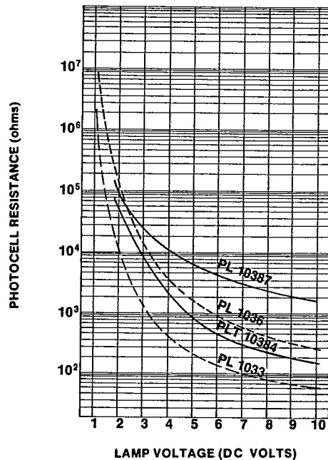
Incandescent Lamp/ Photocell Module Transfer Characteristic
