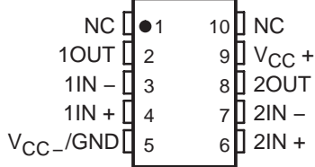
TLV2662M, TLV2262AM U PACKAGE (TOP VIEW)
