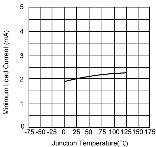
Figure 5. Minimum Load Current vs. Temperature
