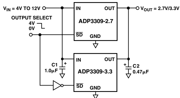
Figure 3. Crossover Switch
