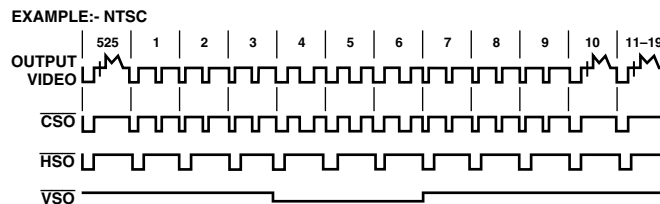
Figure 14. \overline{CSO} , \overline{HSO} , \overline{VSO} Timing Diagram
