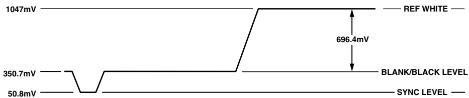
Figure 100. PAL Luma Video Levels
