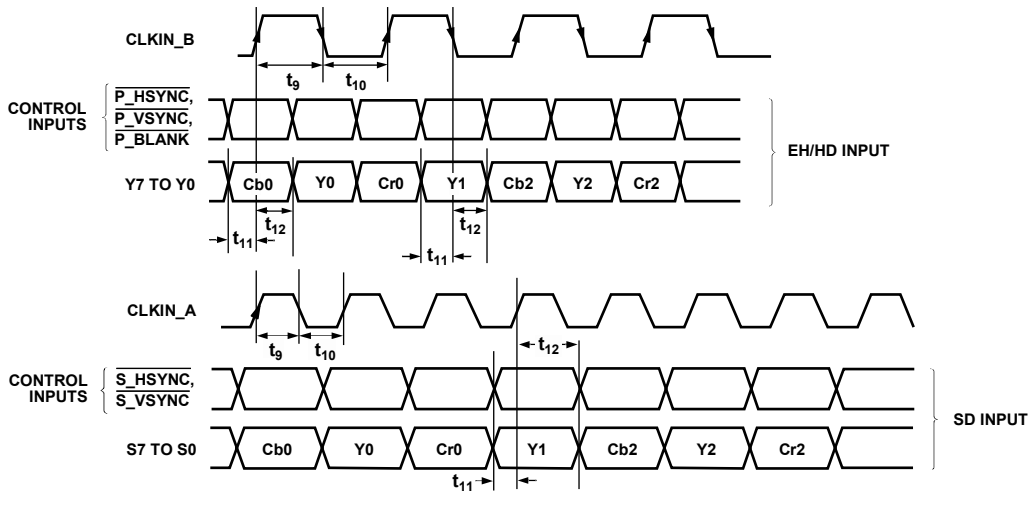
Figure 11. SD and ED/HD-DDR, 8-Bit, 4:2:2 ED/HD and 8-Bit, SD Pixel Input Mode (Input Mode 100)
