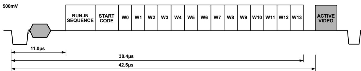
Figure 98. WSS Waveform Diagram
