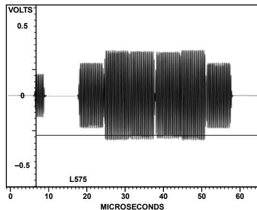
Figure 133. PAL Chroma
