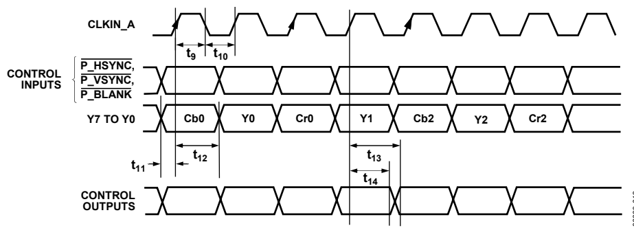
Figure 12. ED Only (at 54 MHz), 8-Bit, 4:2:2 YCrCb (HSYNC/VSYNC) Pixel Input Mode (Input Mode 111)
