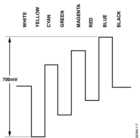
Figure 116. Pb Levels—NTSC
