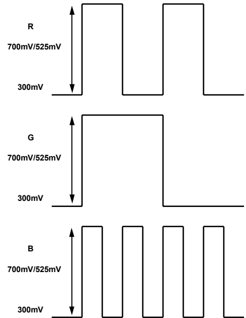
Figure 126. HD RGB Output Levels—RGB Sync Disabled
