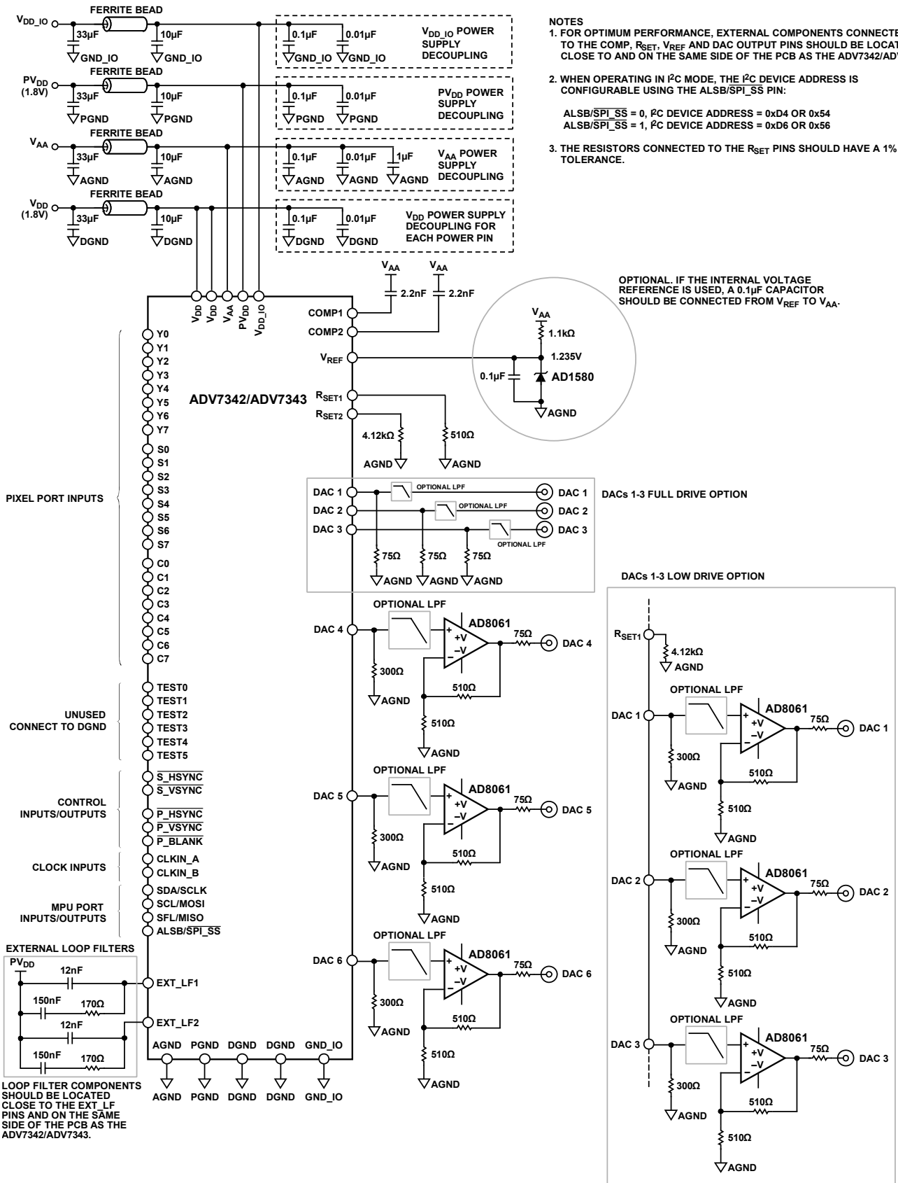
Figure 90. ADV7342/ADV7343 Typical Application Circuit
