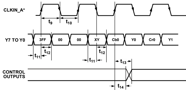
Figure 9. ED/HD-DDR Only, 8-Bit, 4:2:2 YCrCb (EAV/SAV) Pixel Input Mode (Input Mode 010)
