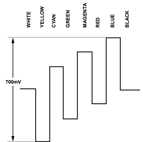
Figure 119. Pb Levels—PAL
