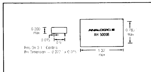
Figure 6. AH50008 Mechanical.
