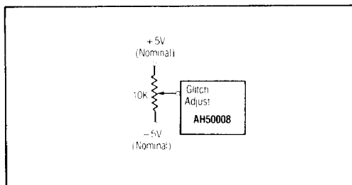
Figure 3. Glitch Adjust.
