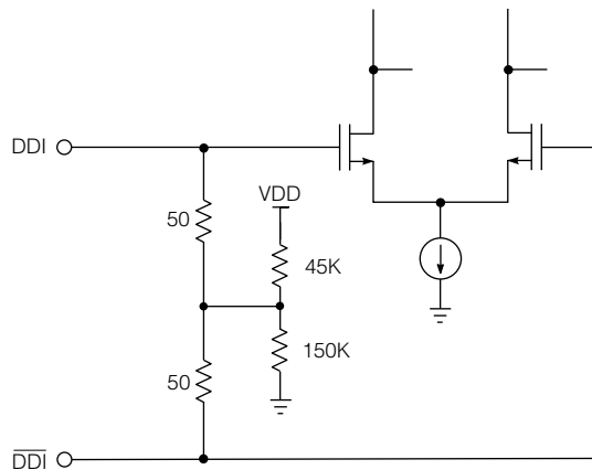
Figure 2 Serial Digital Input
