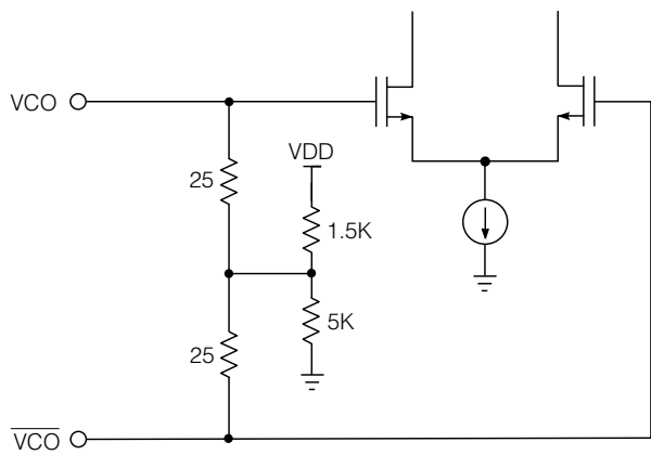
Figure 3 VCO Input
