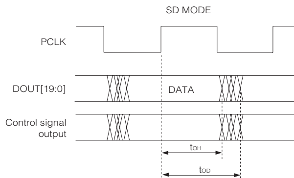
Figure 14 SD PCLK to Data Timing
