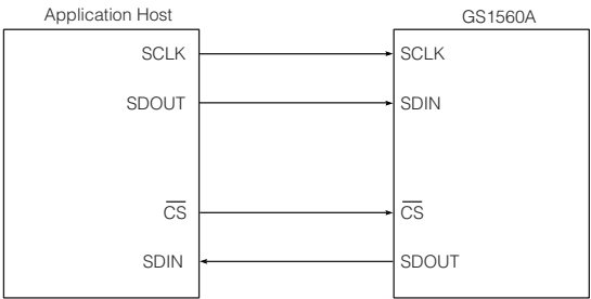
Figure 15 Genum Serial Peripheral Interface (GSPI)
