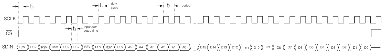
Figure 19 GSPI Write Mode Timing
