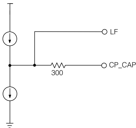
Figure 6 VCO Control Output & PLL Lock Time Capacitor
