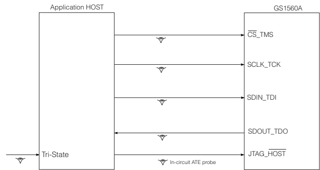
Figure 21 System JTAG
