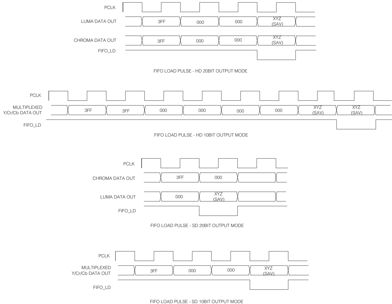
Figure 11 \overline{\text{FIFO\_LD}} Pulse Timing
