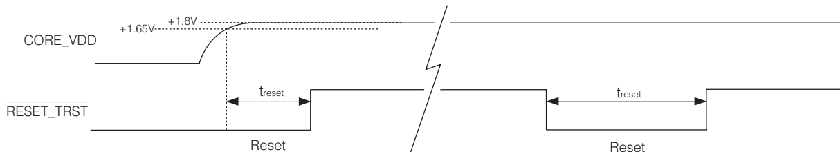
Figure 22 Reset Pulse
