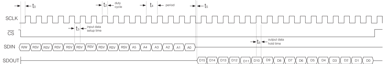
Figure 18 GSPI Read Mode Timing
