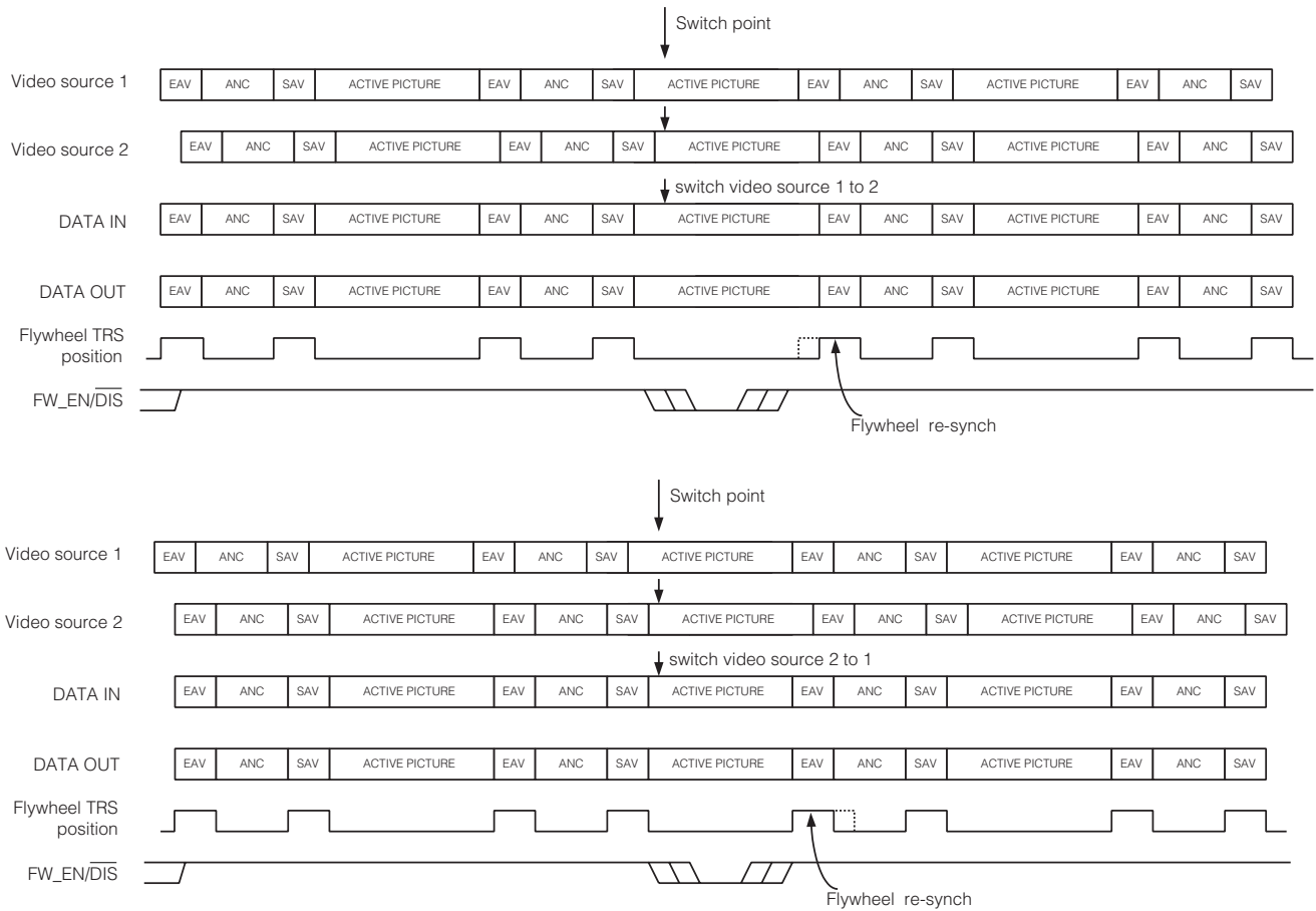
Figure 8 Switch Line Locking
