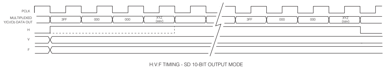
Figure 9 H, V, F Timing
