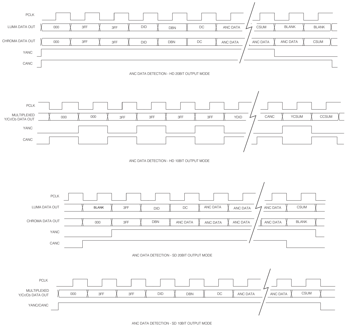
Figure 12 YANC and CANC Output Signal Timing
