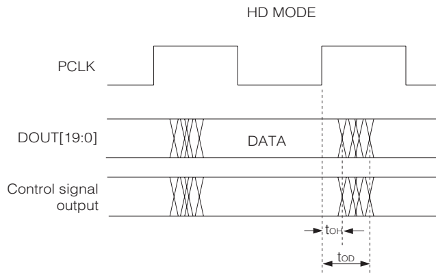
Figure 13 HD PCLK to Data Timing
