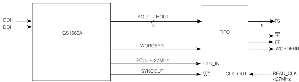
Figure 10 DVB-ASI FIFO Implementation using the GS1560A
