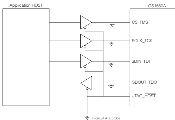
Figure 20 In-Circuit JTAG
