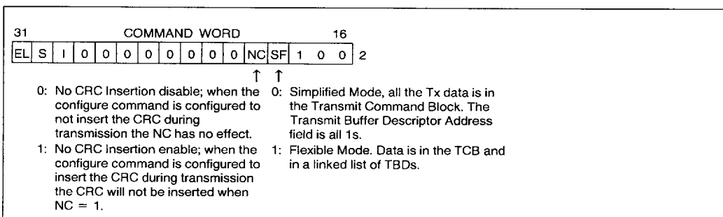
Figure 30. TRANSMIT—Linear Mode
