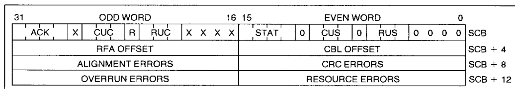
Figure 18. SCB—82586 Mode
