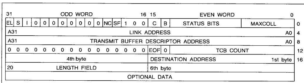
Figure 30. TRANSMIT—Linear Mode
