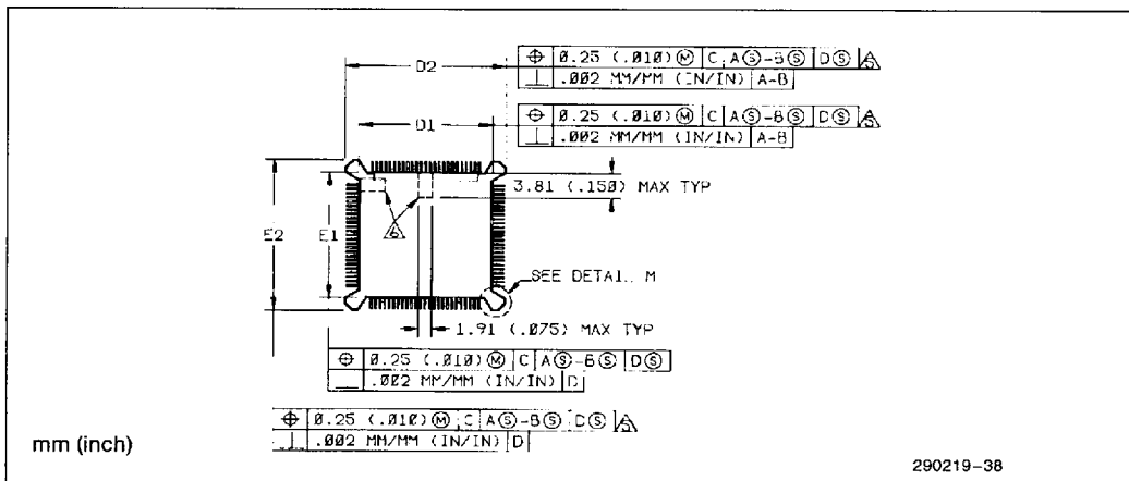
Figure 62. Molded Details
