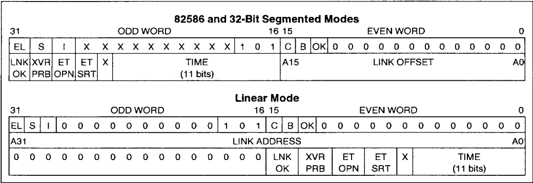
Figure 32. TDR
