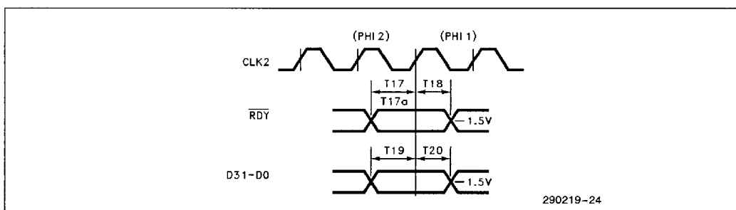
Figure 51. Input Setup and Hold Time
