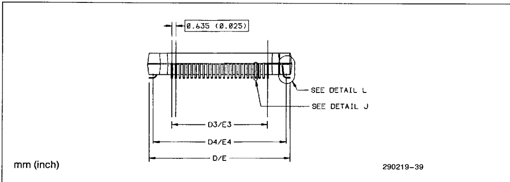
Figure 63. Terminal Details
