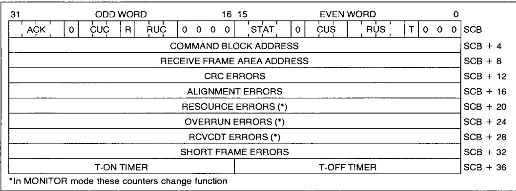
Figure 20. SCB—Linear Mode
