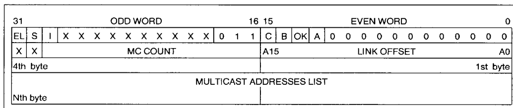
Figure 26. MC Setup—82586 and 32-Bit Segmented Modes
