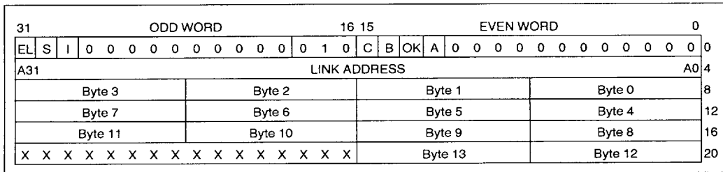
Figure 25. CONFIGURE—Linear Mode
