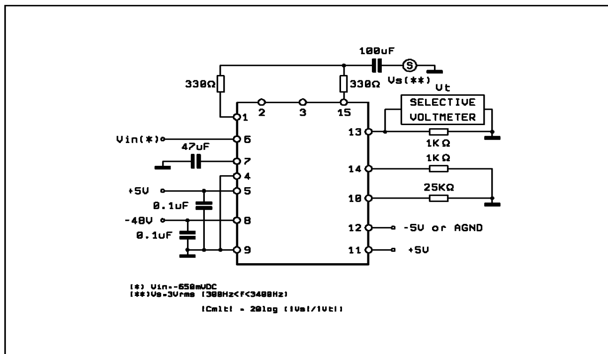
Figure 8: Common Mode Rejection Transversal to Longitudinal
