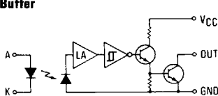
OPB961/OPB971 (Open-Collector Output) Buffer
