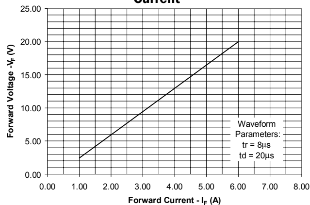
Forward Clamping Voltage vs. Peak Pulse Current Current
