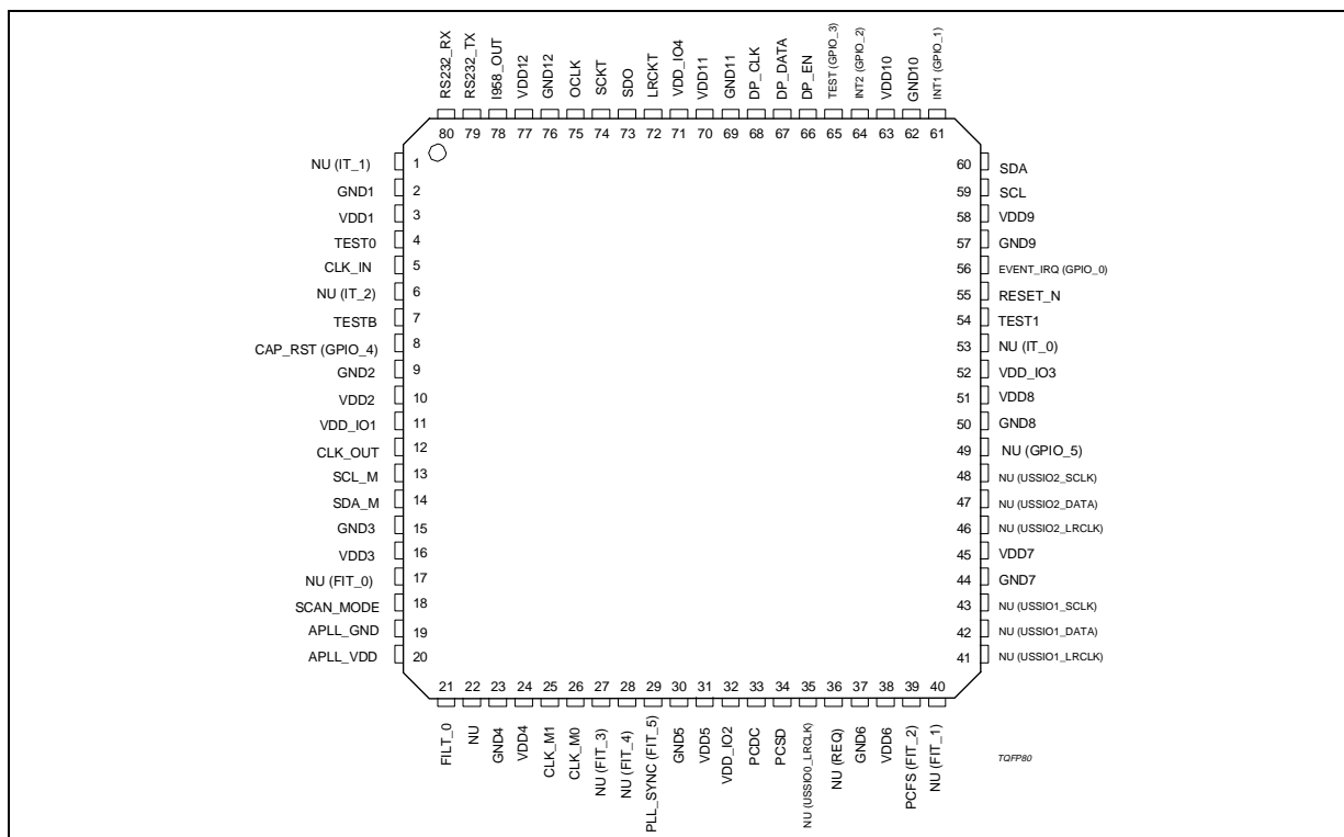
Figure 2. Pin Connection
