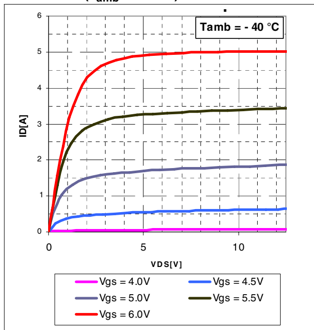
Figure 4. DC output characteristics ( T_{amb} = -40\text{ }^{\circ}\text{C} )
