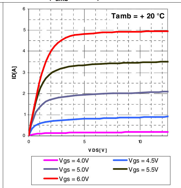
Figure 5. DC output characteristics ( T_{amb} = 20\text{ }^{\circ}\text{C} )
