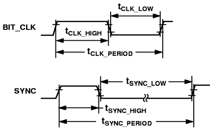
Figure 3. Clock Timing
