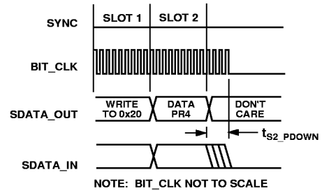
Figure 6. AC Link, Link Low Power Mode Timing
