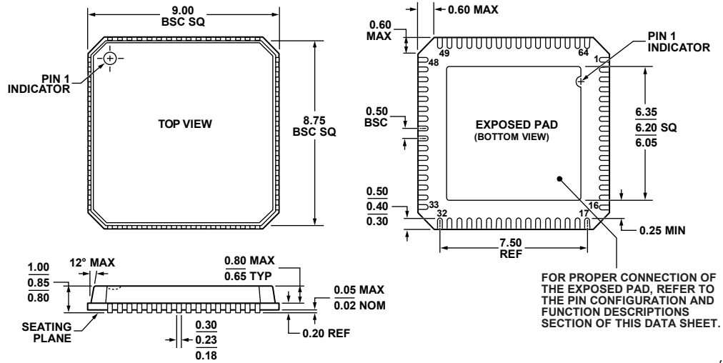
COMPLIANT TO JEDEC STANDARDS MO-220-VMMD-4 Figure 46. 64-Lead Lead Frame Chip Scale Package [LFCSP_VQ] 9 mm × 9 mm Body, Very Thin Quad (CP-64-4) Dimensions shown in millimeters
