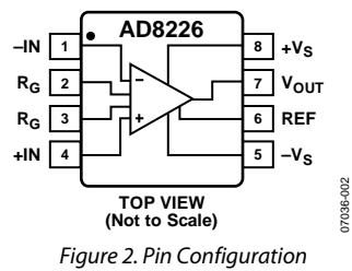
Figure 2. Pin Configuration
