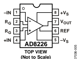
Figure 5. Pinout Diagram
