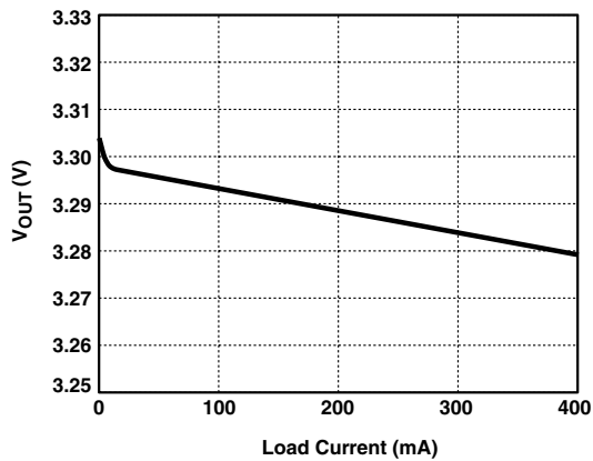
Figure 5. Load Regulation
