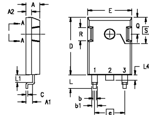
TO-247 SMD Outline
