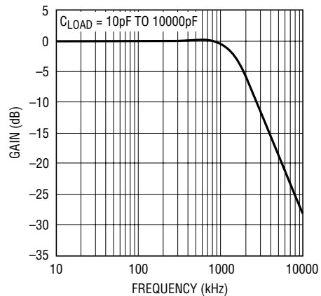
V OCM Gain vs Frequency, V S = ±2.5V
