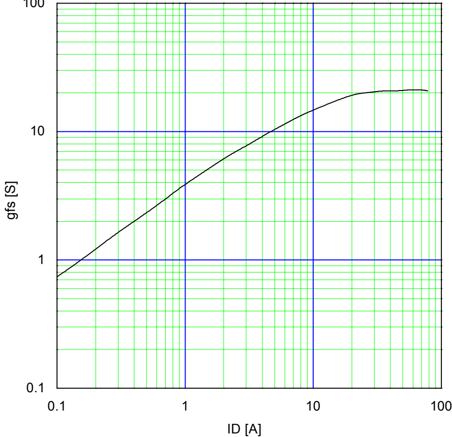
Typical Transconductance g_{fs}=f(I_D):80\text{ }\mu\text{s pulse test, }V_{DS}=25\text{V, }T_{ch}=25^\circ\text{C}
